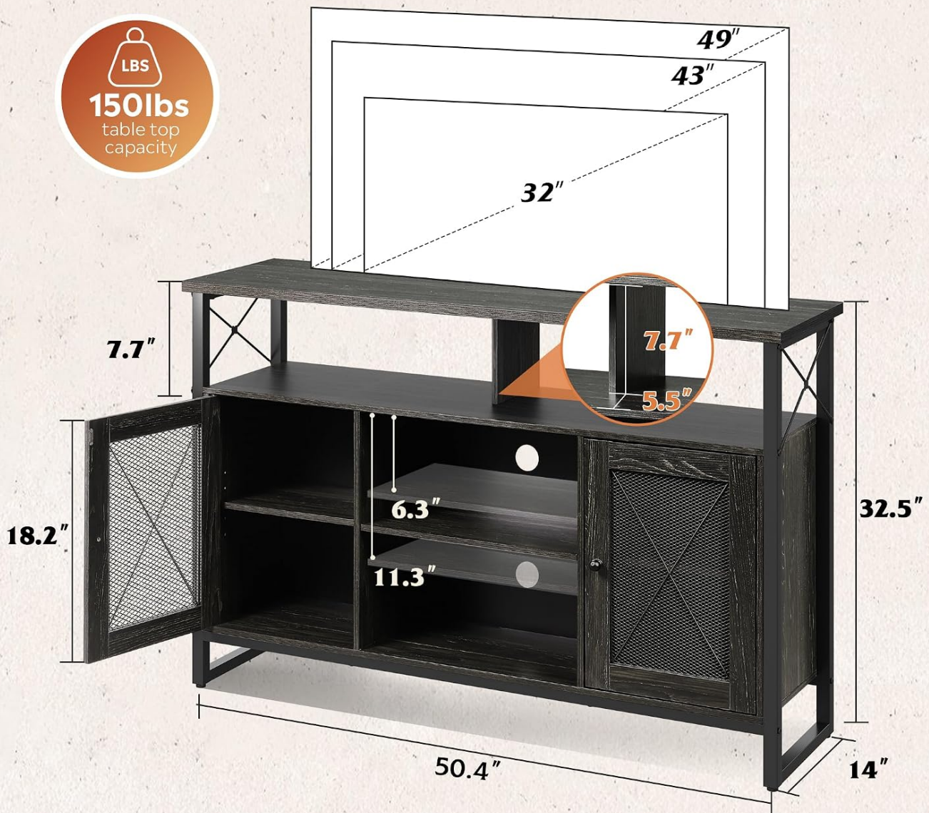
Image 4.1: Product dimensions and TV size compatibility. The stand measures 50.4" W x 14" D x 32.5" H.
