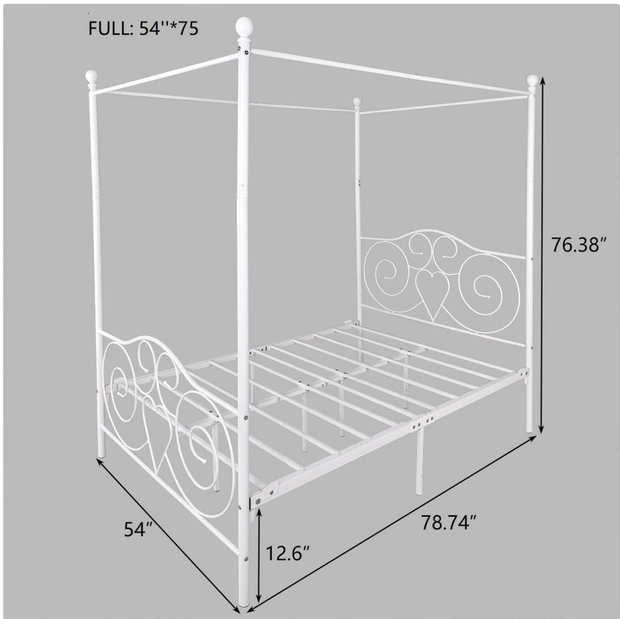
Figure 8.1: Detailed dimensions of the Albearing Full Canopy Bed Frame.
