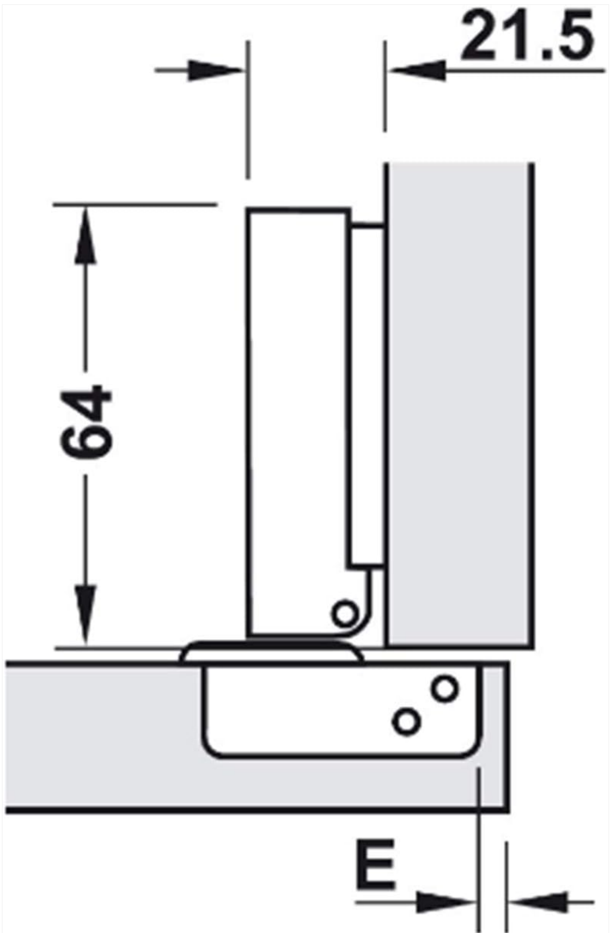
Image Description: A side-view diagram showing a cabinet door installed with a hinge in a corner stop configuration. Key dimensions are indicated: 21.5mm for the door thickness, 64mm for the hinge arm length, and 'E' for the cup distance from the cabinet edge.
