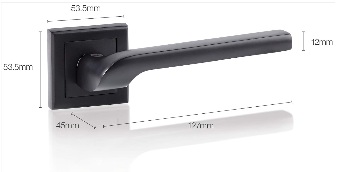
Image: Detailed dimensions of the Yale Siena door handle, showing handle length (127mm), rose size (53.5mm x 53.5mm), and handle projection (45mm).
