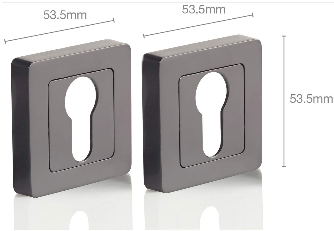
Image: Dimensions of the square keyhole covers, each measuring 53.5mm x 53.5mm.
