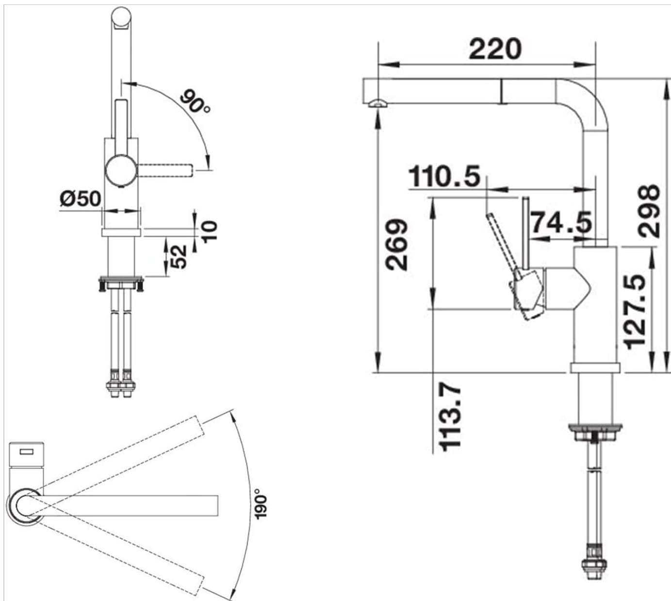
Figure 3: Technical drawing showing the dimensions and swivel range of the BLANCO Lanora-S-F faucet.
