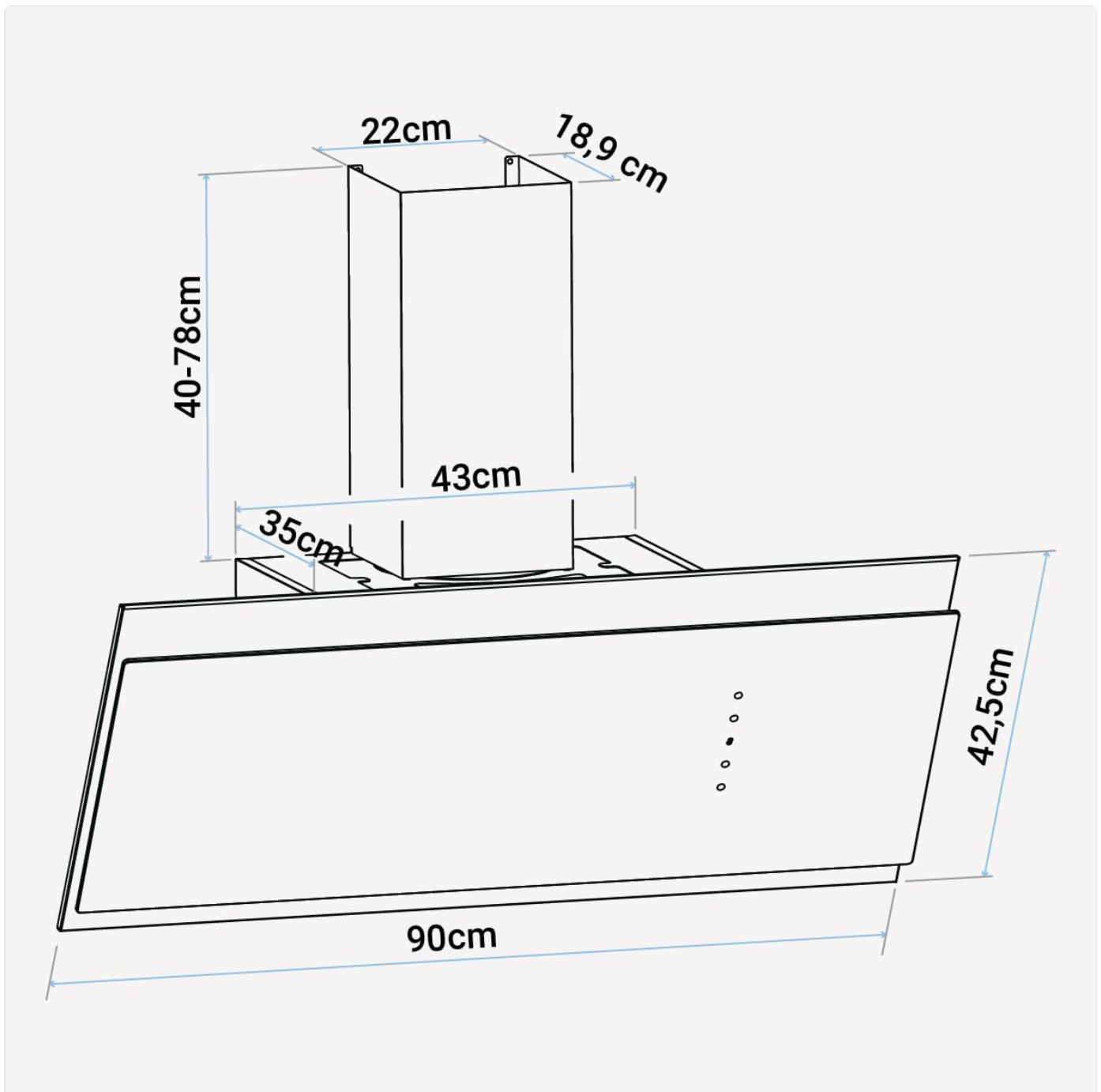
Image: Technical diagram illustrating the dimensions of the range hood, including width (90cm), height, and depth, along with chimney measurements.
