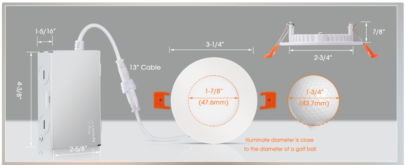
Image 4.1: Visual guide for the installation process, from cutting the hole to securing the fixture.
