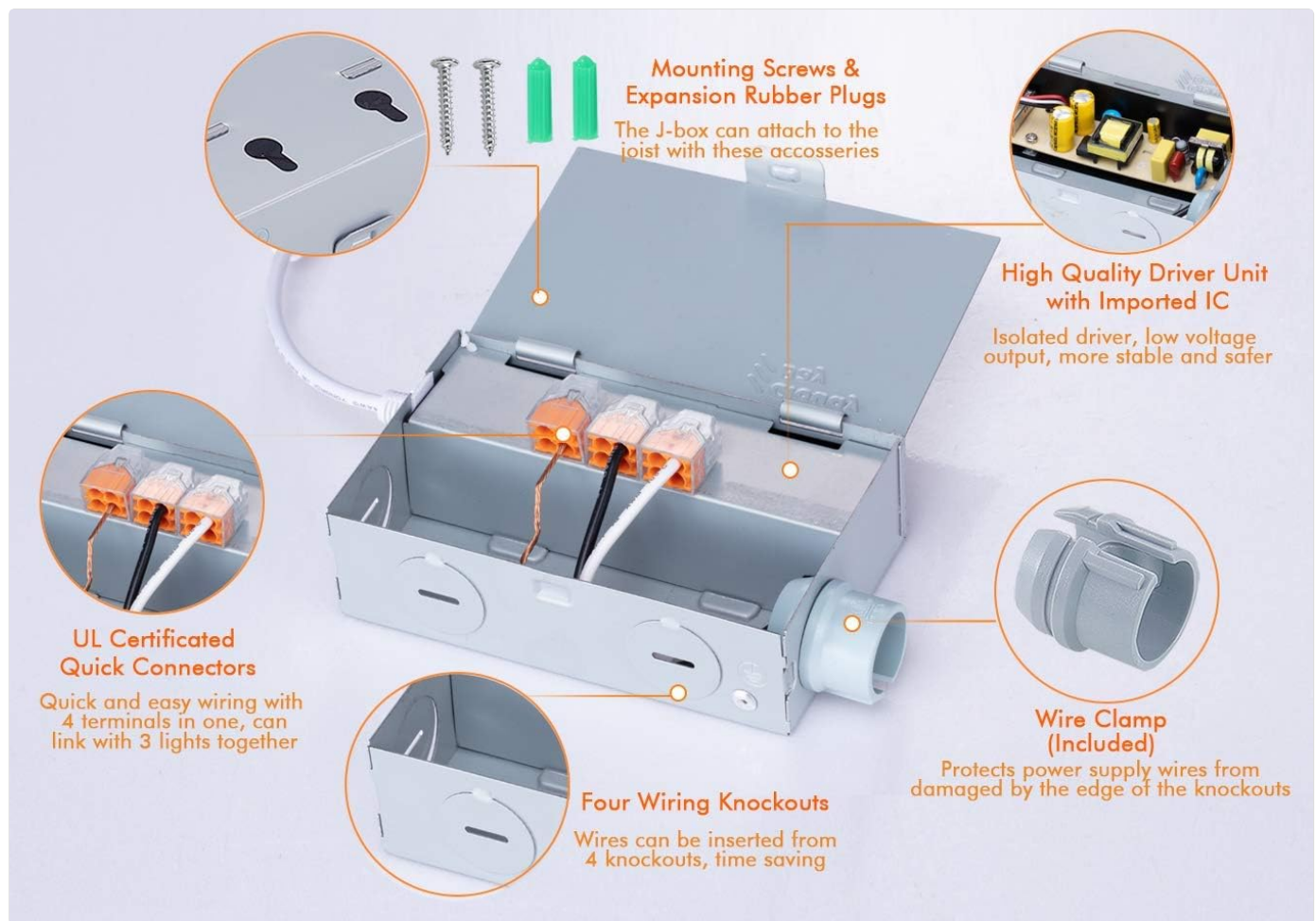
Image 4.2: Close-up of the junction box showing quick connectors for easy and secure wiring.
