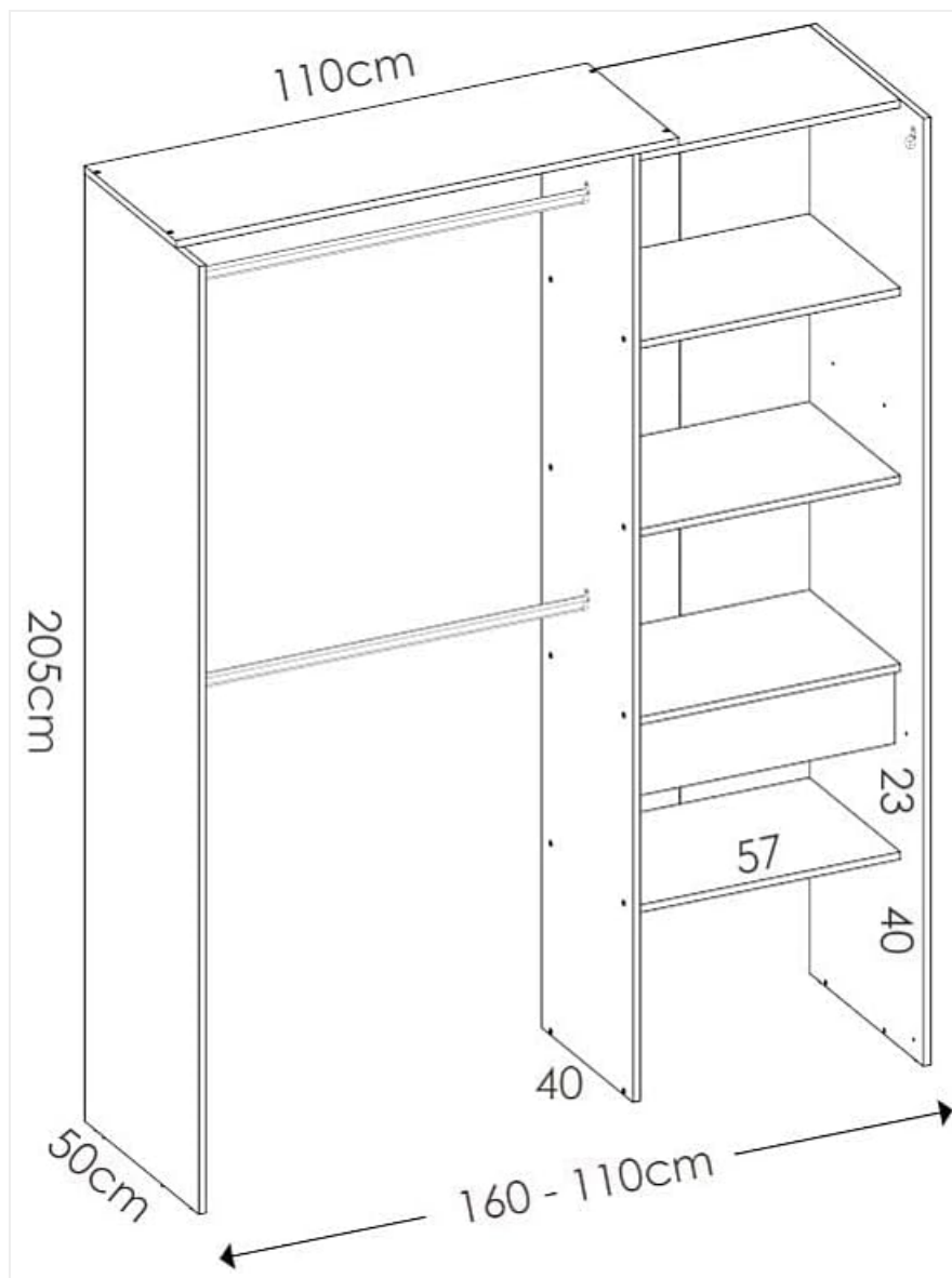
Figure 2: Technical drawing showing dimensions and adjustable width (110-160 cm).
