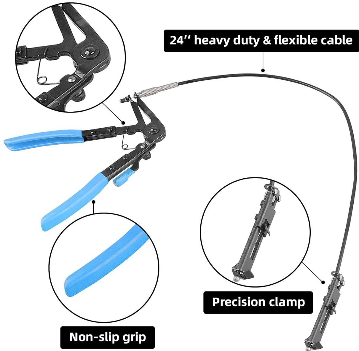
Figure 5: Flexible Hose Clamp Plier with detailed views of its features.
