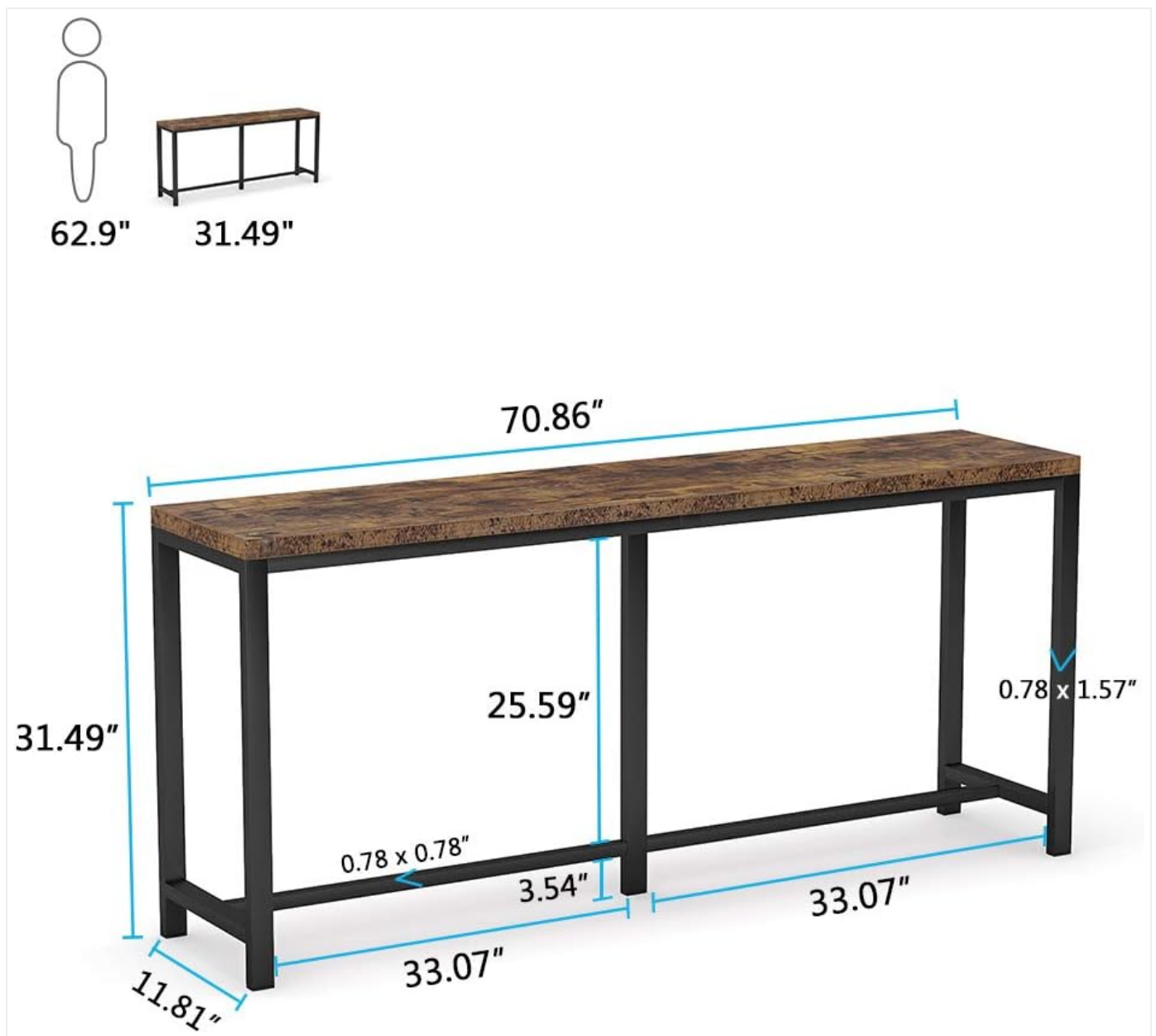
Figure 1: Product Dimensions and Components Overview
