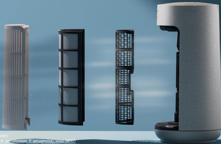
Figure 4: Filter components and their placement within the unit.
