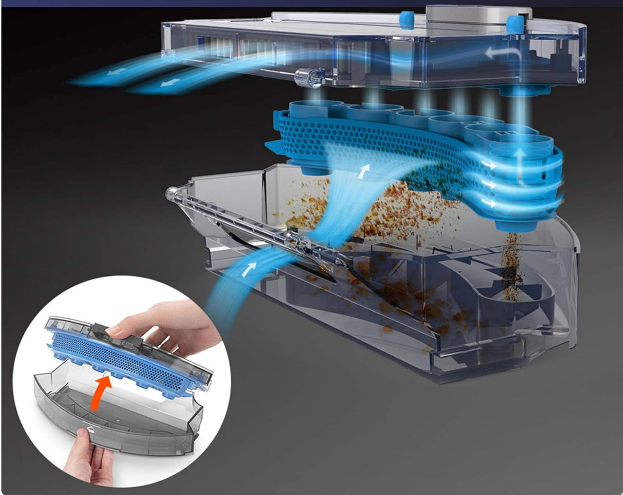
Image: An exploded view diagram illustrating the components of the ILIFE A80 Max's cellular dustbin and its airflow path for efficient filtration.
