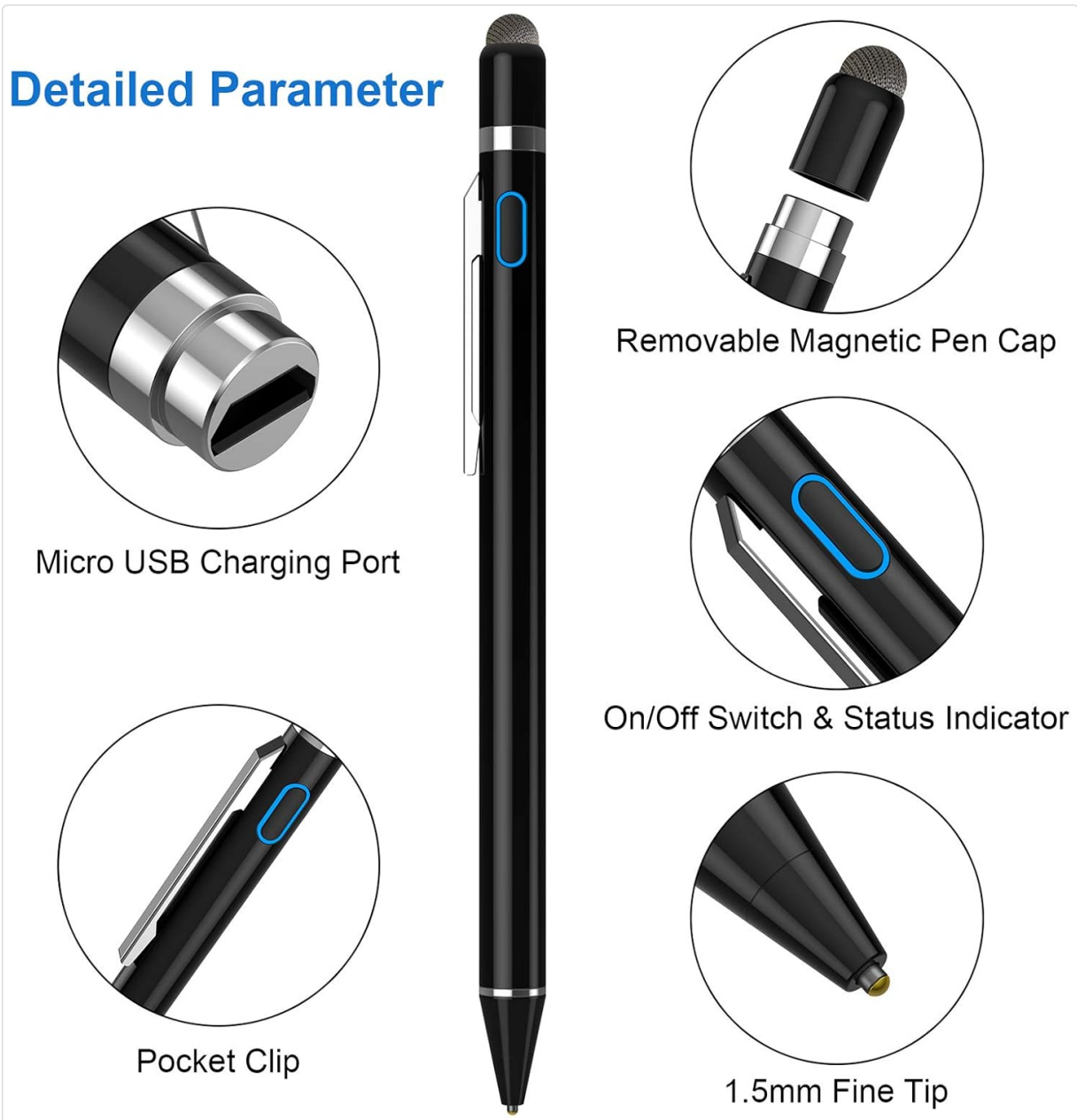
Image 2.1: Detailed view of the NTHJOYS stylus, highlighting its Micro USB charging port, On/Off switch with status indicator, removable magnetic pen cap, pocket clip, and 1.5mm fine tip.
