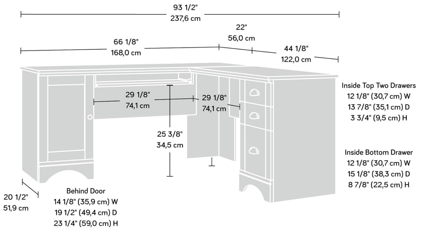
Image 2.3: Detailed dimensions of the Sauder Harbor View Corner Computer Desk, including measurements for the desktop, drawer interiors, and cabinet space.
