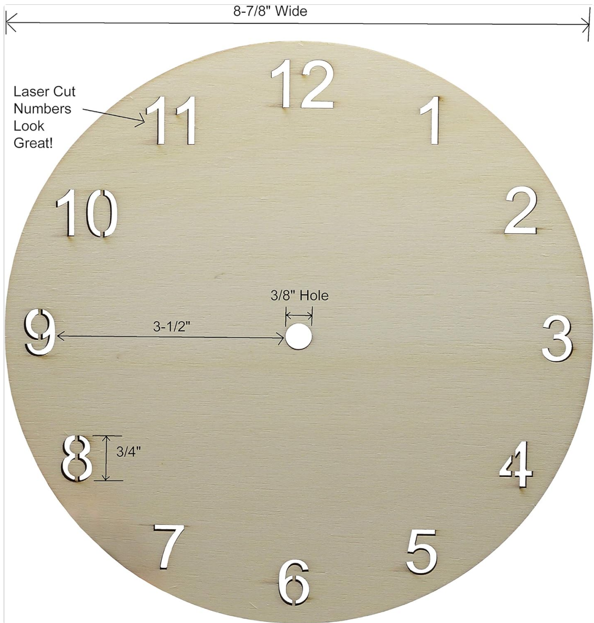
Image: Creative Hobbies Clock Face with Key Dimensions. This image illustrates the clock face with measurements for its width (8-7/8" wide) and the 3/8" center hole, along with a note about the laser-cut numbers.
