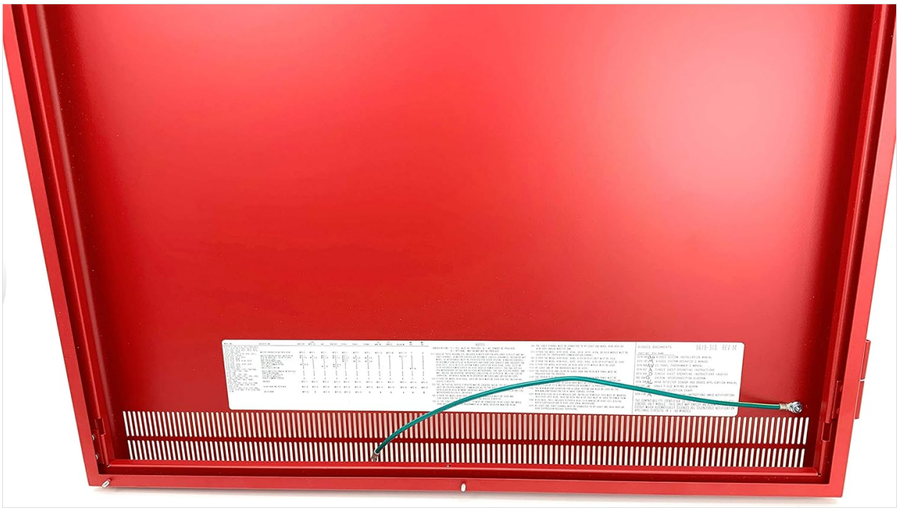
Figure 1: Internal view of the 3-bay red enclosure, illustrating the layout for component installation and internal wiring pathways.
