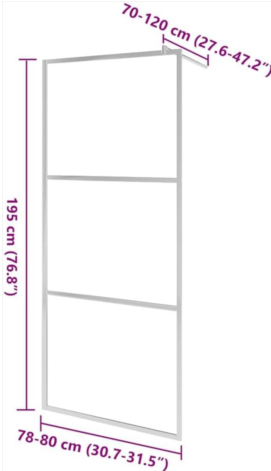
Image: Dimensional diagram of the shower wall, indicating height (195 cm / 76.8") and width (78-80 cm / 30.7-31.5"), and adjustable support bar length (70-120 cm / 27.6-47.2").
