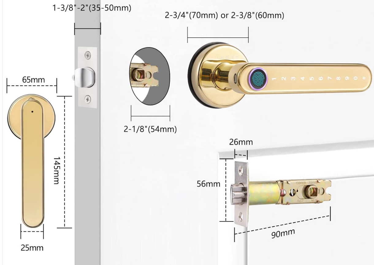
Figure 4: Installation diagram with dimensions.
