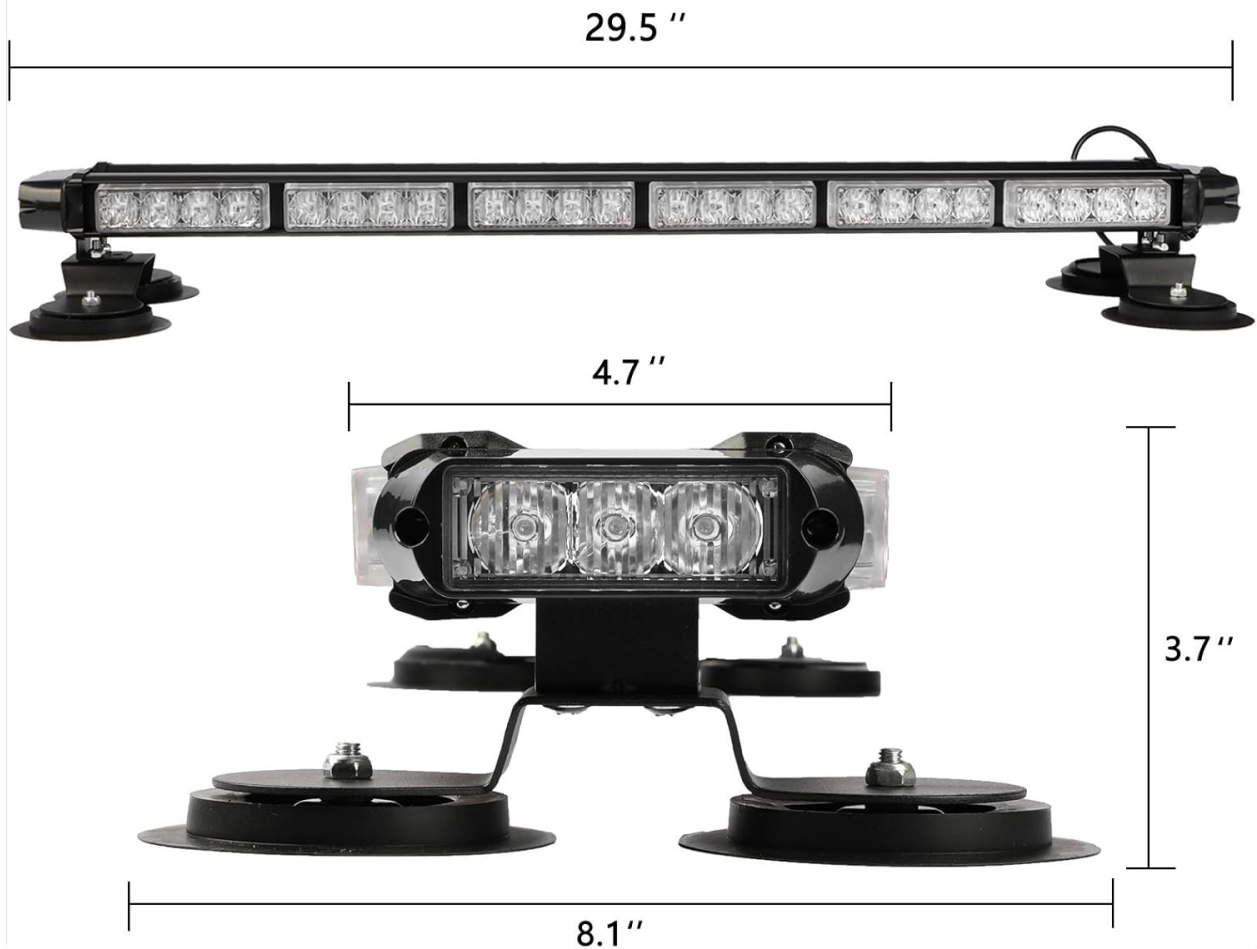
Figure 6: Product Dimensions
