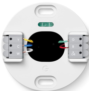
Image: The backplate of the Nest Thermostat showing the wiring terminals (Y, C, W, G, R, OB) for connecting to your HVAC system.
