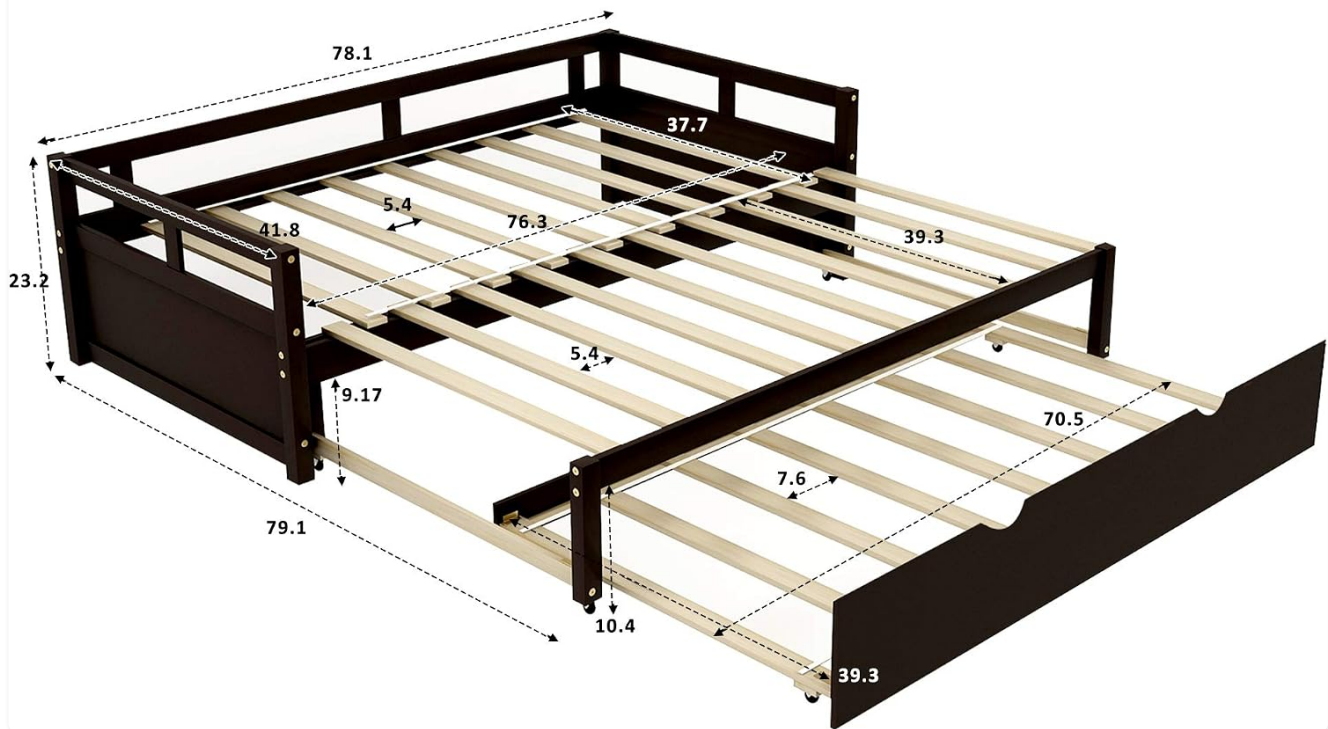
Figure 6: Product Dimensions
