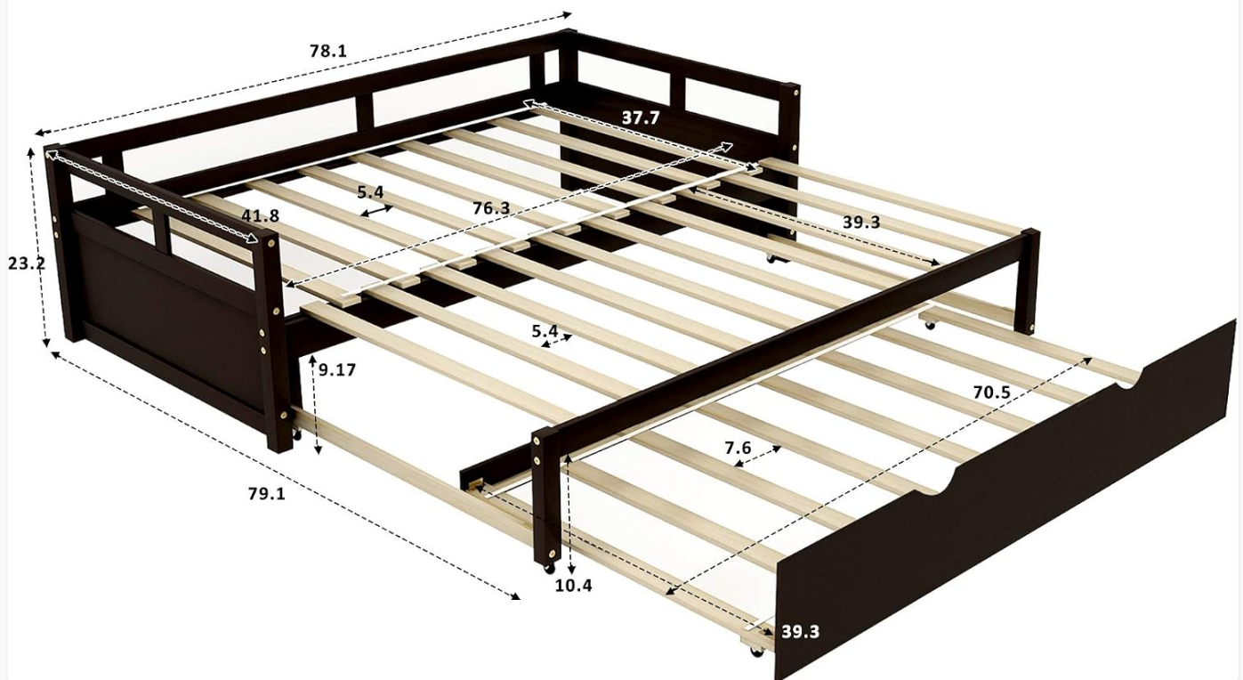
Image: Dimensional drawing of the daybed, illustrating key measurements.
