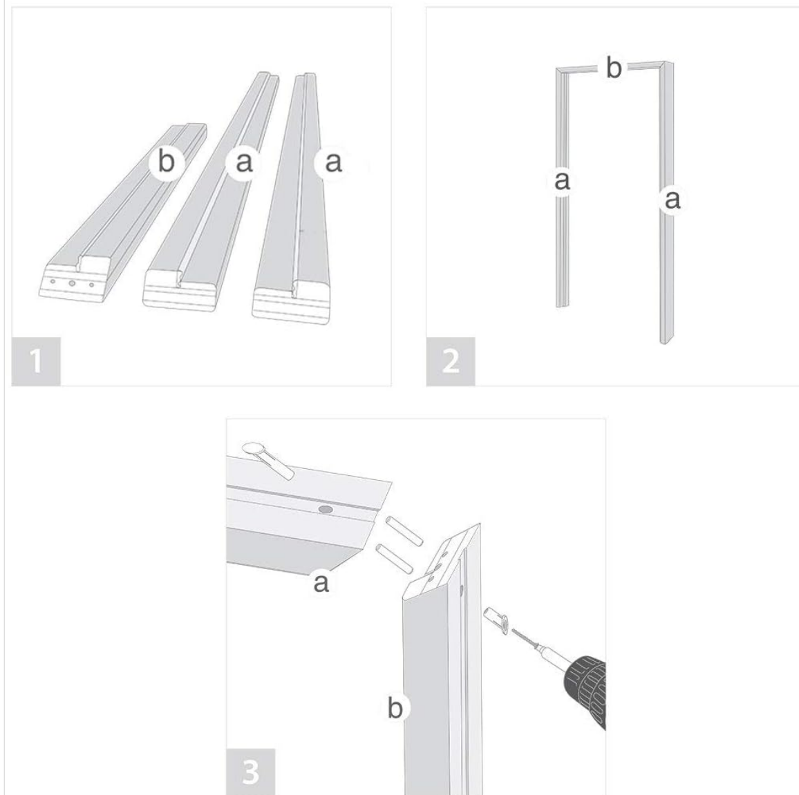
Image: Step-by-step diagram showing the assembly of the door frame components (parts 'a' and 'b') before installation.
