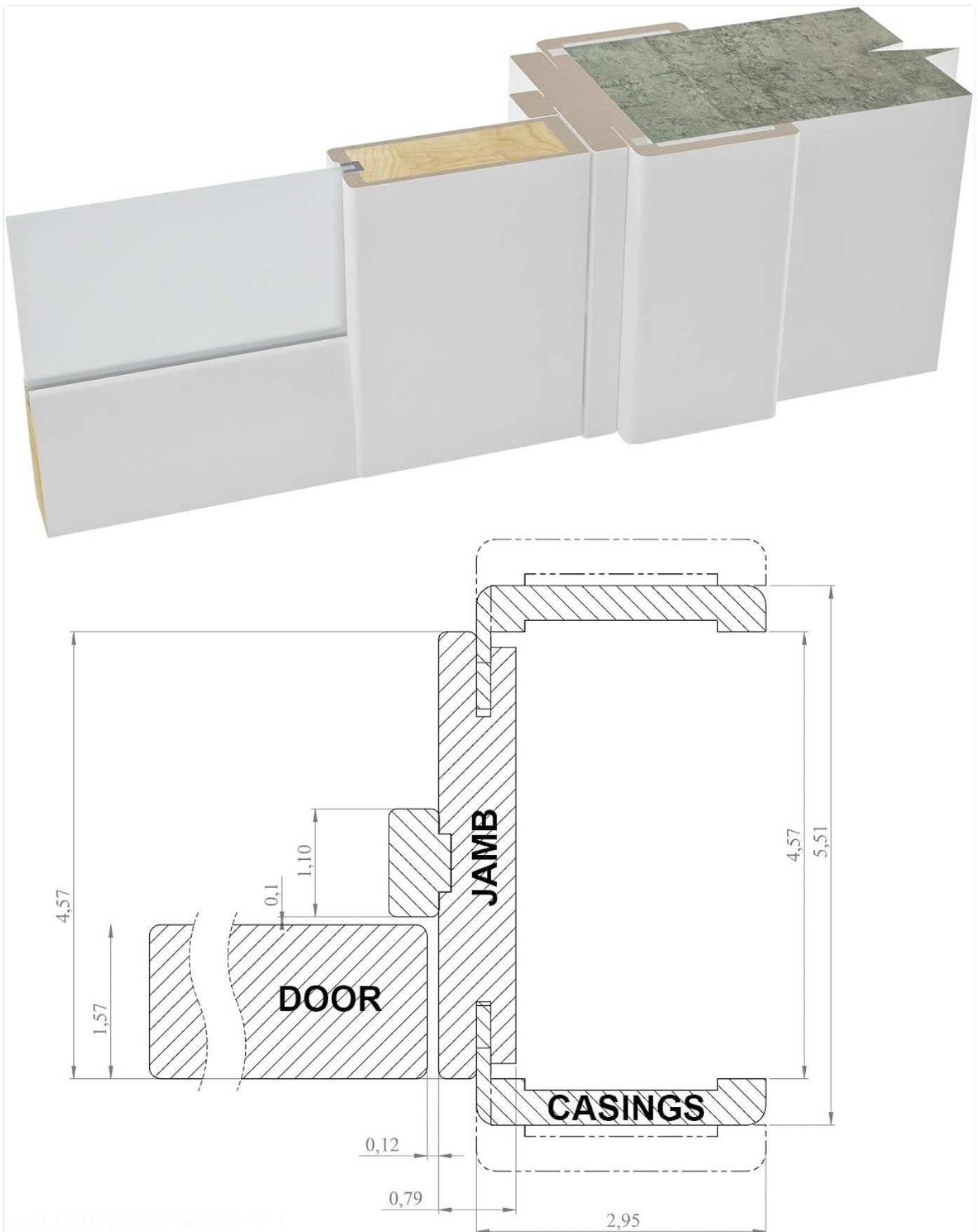
Image: Technical diagram illustrating the cross-section of the door, jamb, and casings with key dimensions.
