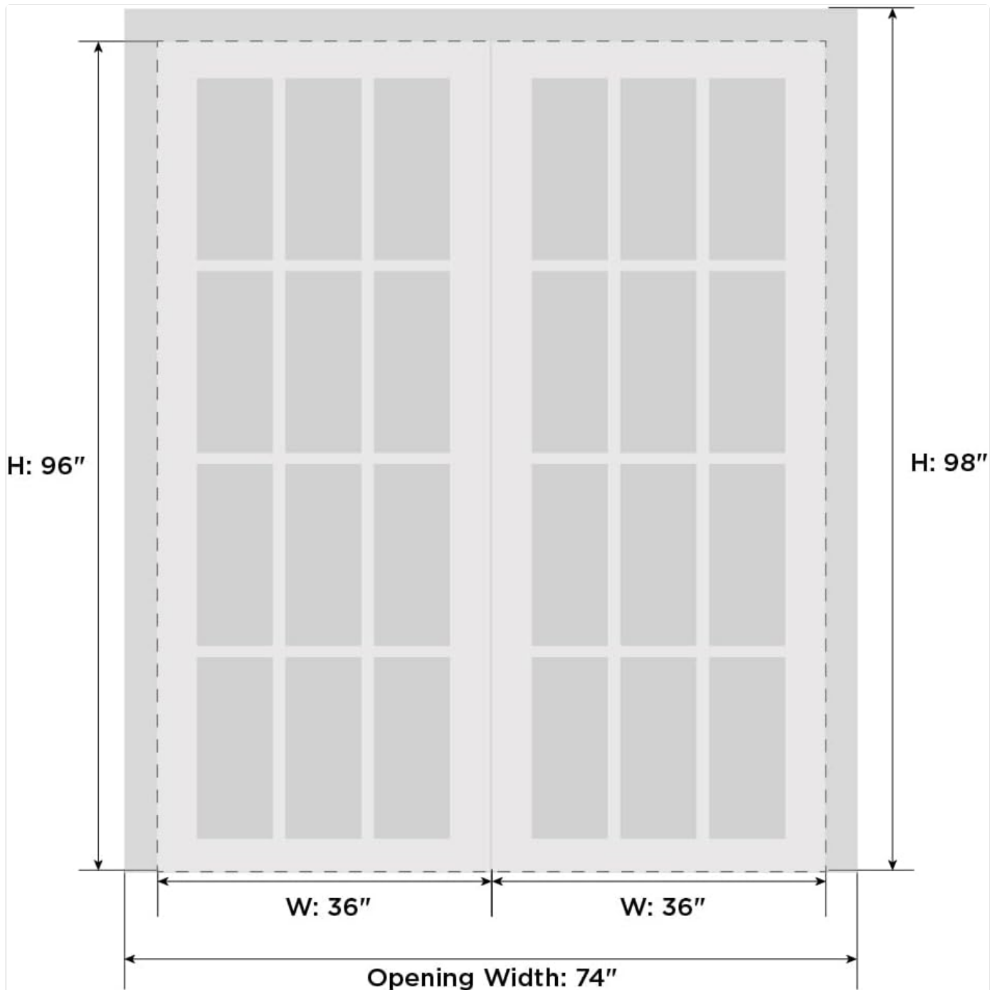
Image: Measurement diagram illustrating the recommended rough opening for the 72" x 96" double doors, showing a 74" width and 98" height for the opening.
