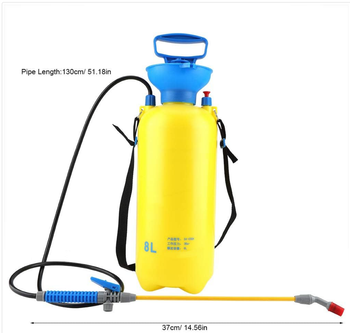
Figure 2.3: The spray wand's blue trigger mechanism, which can be pressed for spraying and pushed forward to lock for continuous operation, along with the adjustable nozzle for spray pattern control.
