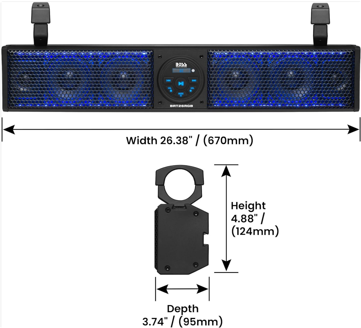
Image: Technical drawing illustrating the width (26.38" / 670mm), height (4.88" / 124mm), and depth (3.74" / 95mm) of the BRT26RGB sound bar, along with a detailed view of the mounting clamp.
