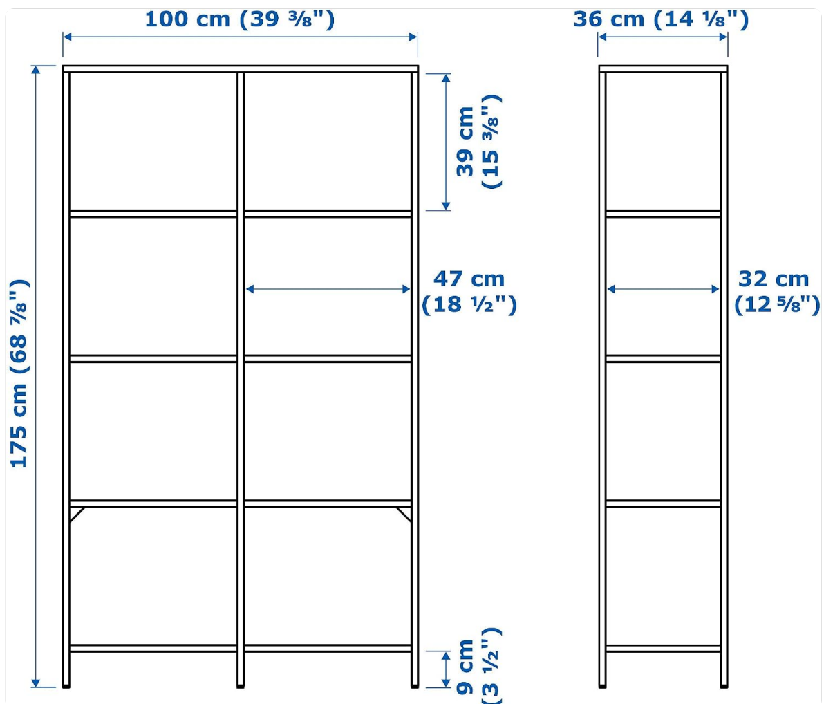
Figure 5: Detailed dimensions of the VITTSJÖ shelf unit, including overall height, width, depth, and individual shelf spacing.
