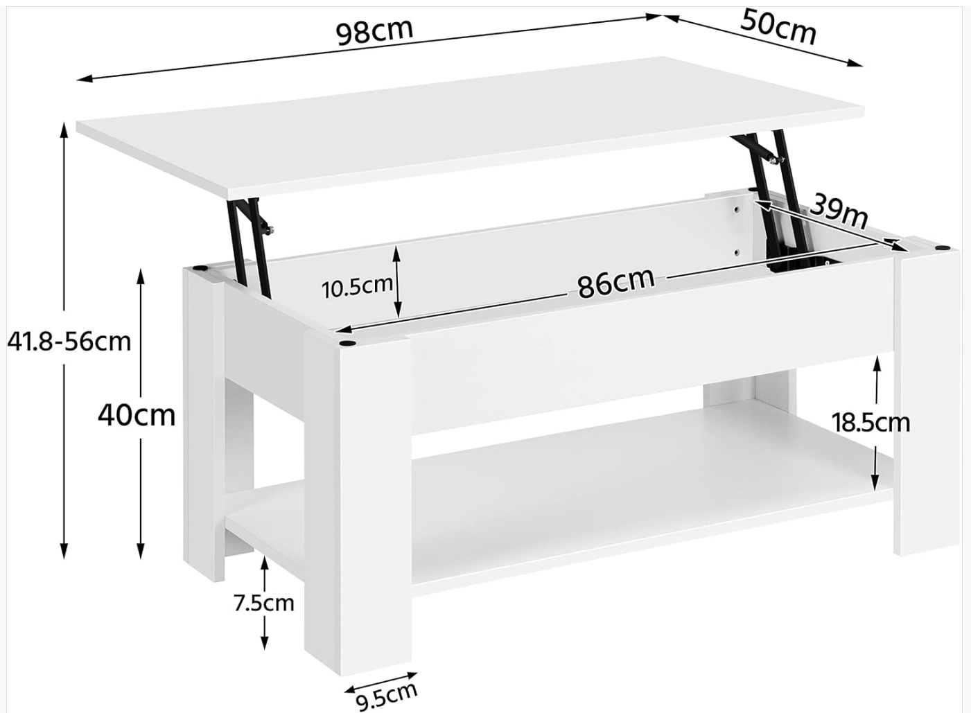
Figure 1: Product Dimensions for reference during assembly.
