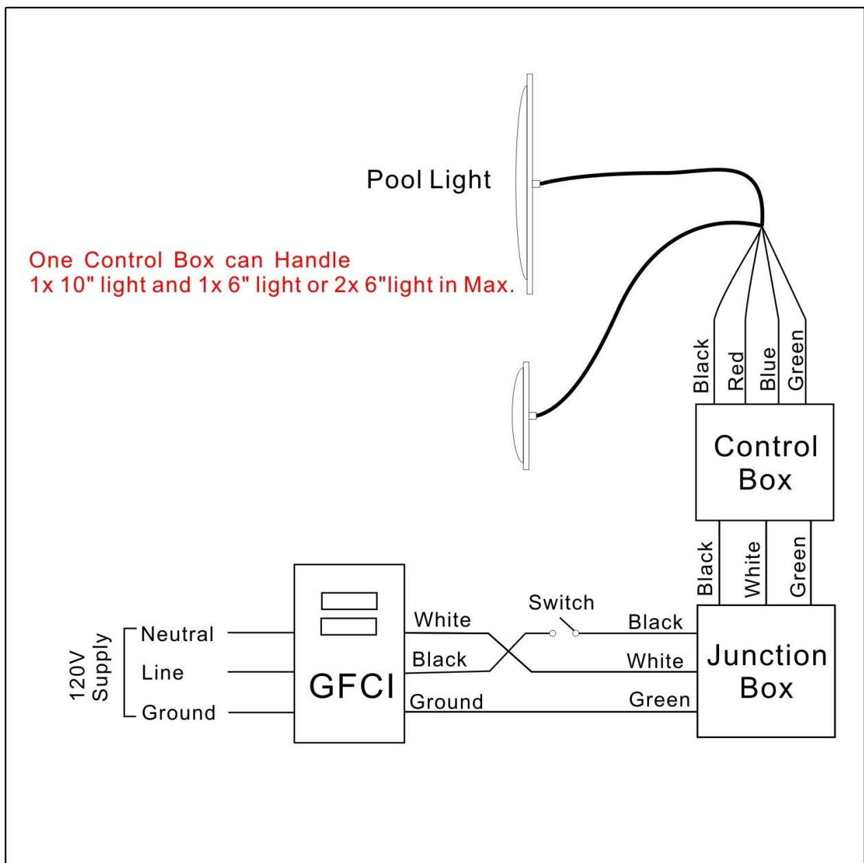
Figure 4: Control box wiring for managing multiple lights.
