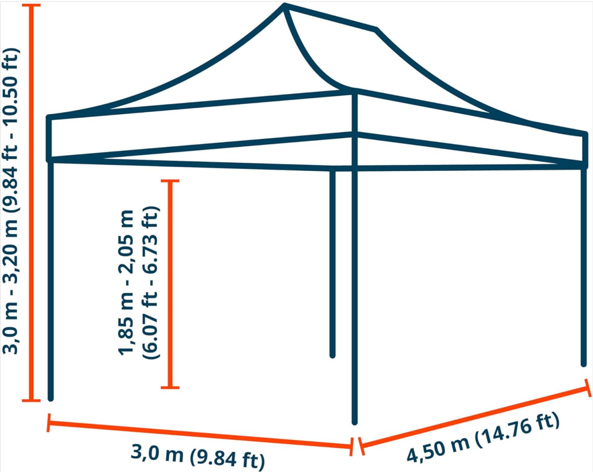
Figure 7.1: Canopy dimensions overview.
