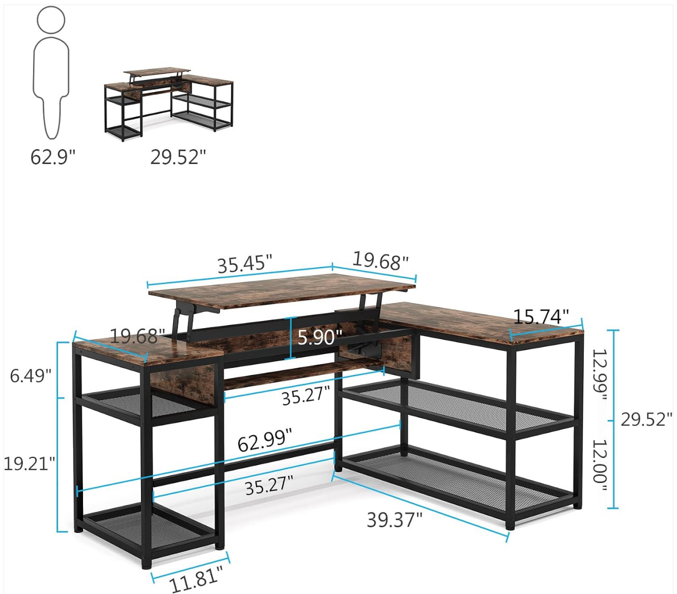
Figure 2: Detailed dimensions of the L-shaped desk, including the lift-top section and storage areas.
