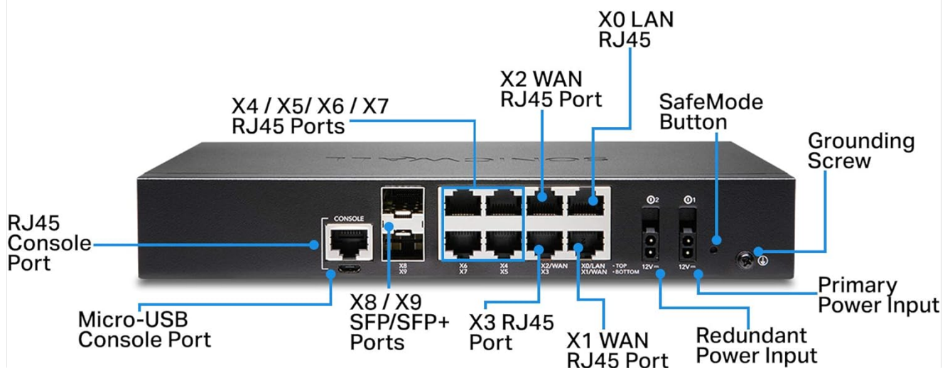
Figure 4: Detailed view of the TZ570 Rear Panel, illustrating the RJ45 Console Port, Micro-USB Console Port, X8 / X9 SFP/SFP+ Ports, X4 / X5 / X6 / X7 RJ45 Ports, X3 RJ45 Port, X2 WAN RJ45 Port, X1 WAN RJ45 Port, X0 LAN RJ45, SafeMode Button, Grounding Screw, Primary Power Input, and Redundant Power Input.
