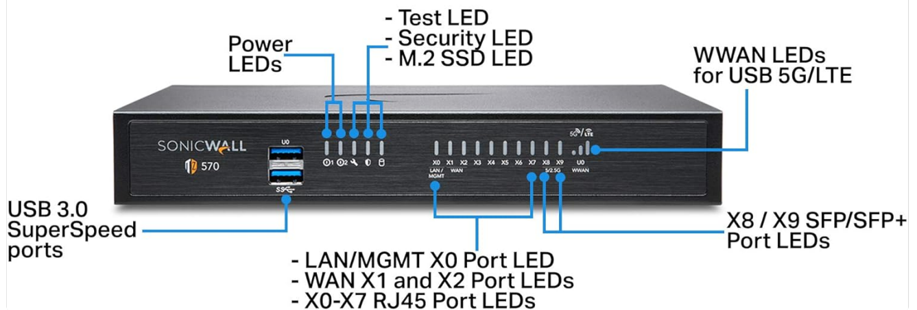
Figure 3: Detailed view of the TZ570 Front Panel, showing USB 3.0 SuperSpeed ports, Power LEDs, Test LED, Security LED, M.2 SSD LED, LAN/MGMT X0 Port LED, WAN X1 and X2 Port LEDs, X0-X7 RJ45 Port LEDs, X8 / X9 SFP/SFP+ Port LEDs, and WWAN LEDs for USB 5G/LTE.
