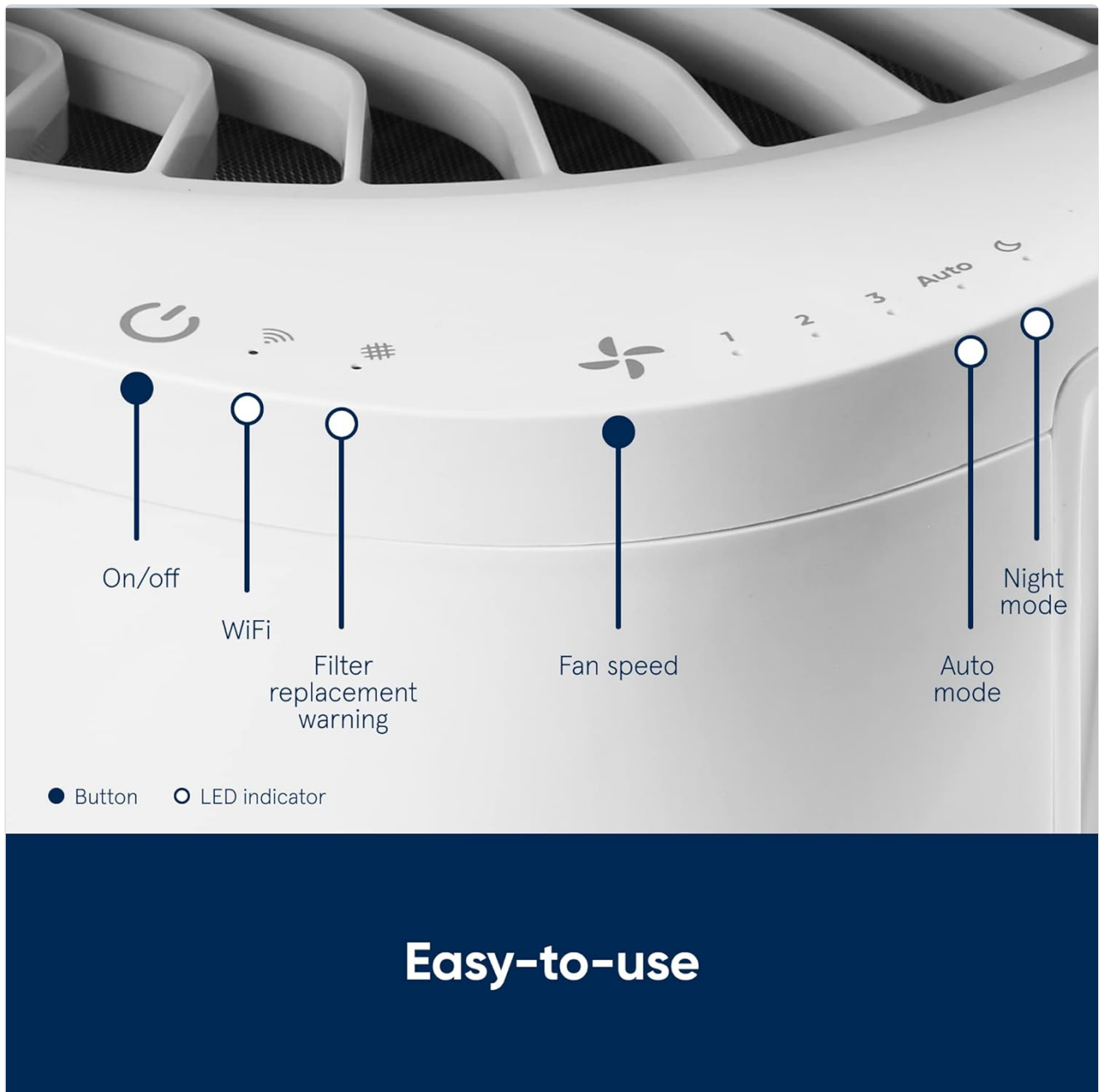
Figure 3.2: Control Panel Layout
