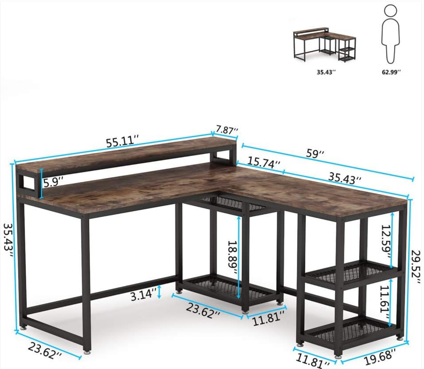
Figure 5: Product Dimensions. Refer to this diagram for detailed measurements of the desk.
