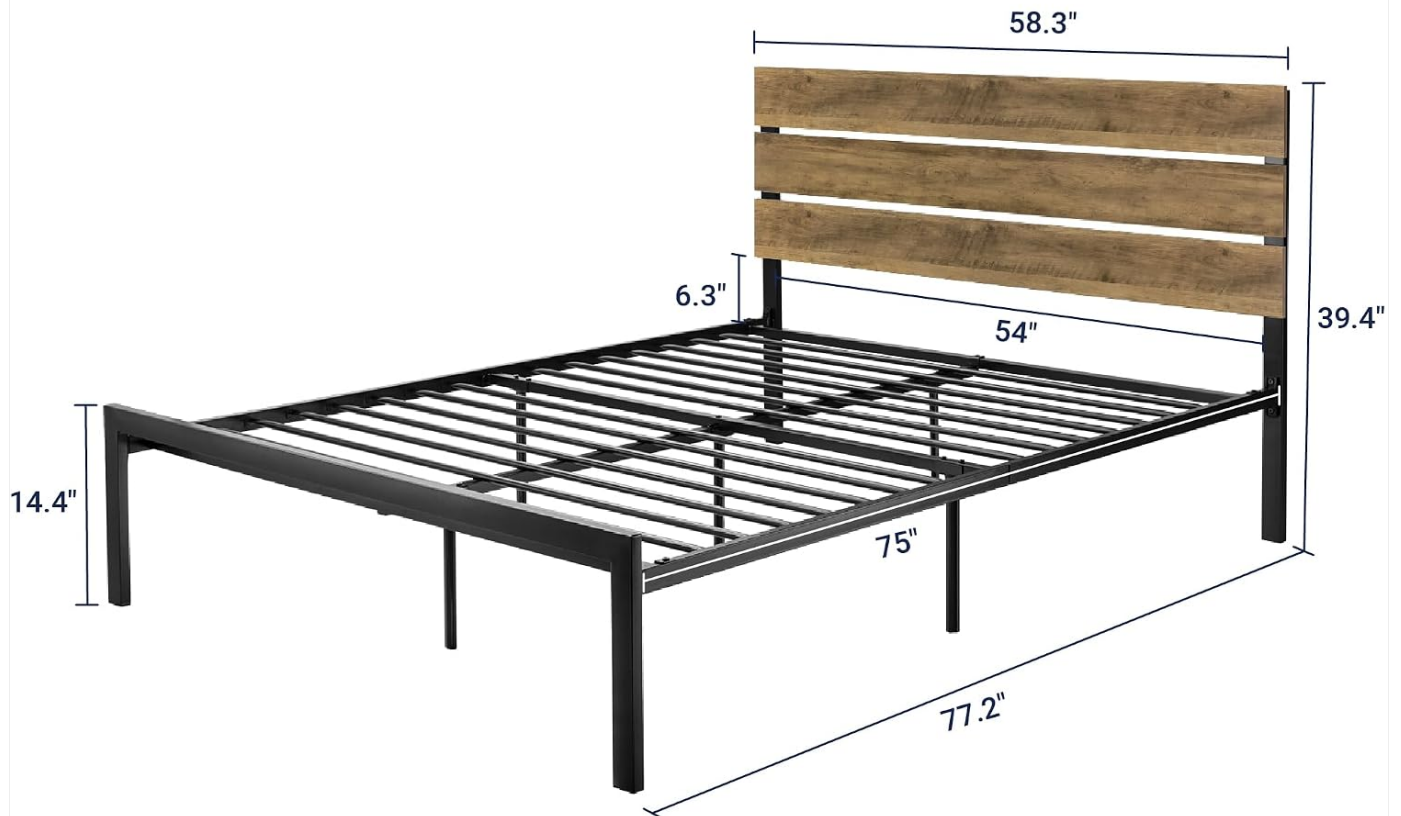
Figure 9: Detailed dimensions of the bed frame.
