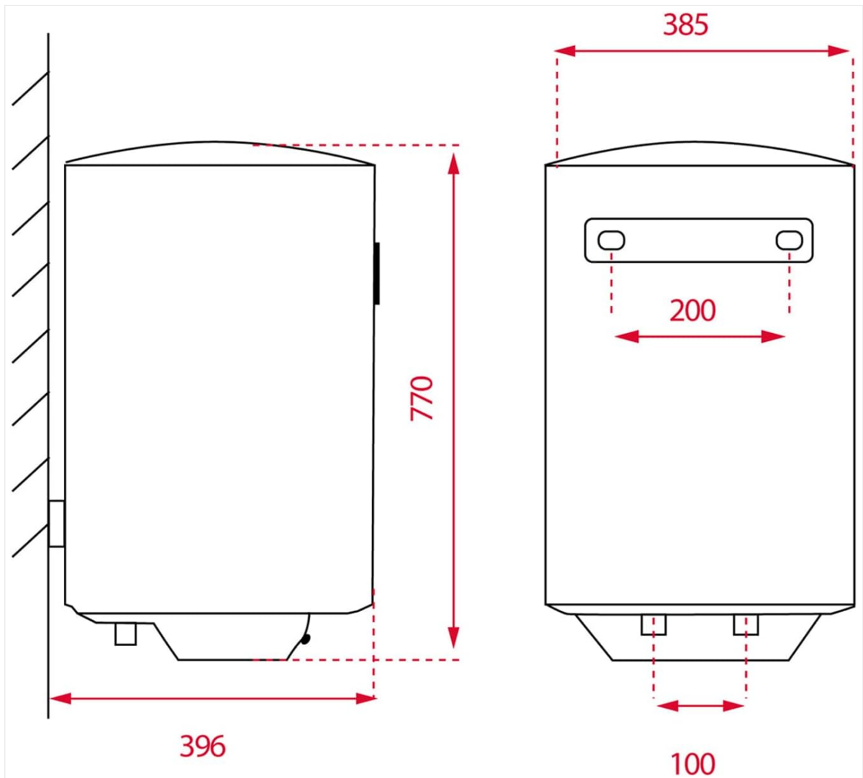
Image 3: Technical drawing illustrating the dimensions (in millimeters) of the Teka EWH 50 C electric water heater for vertical installation.
