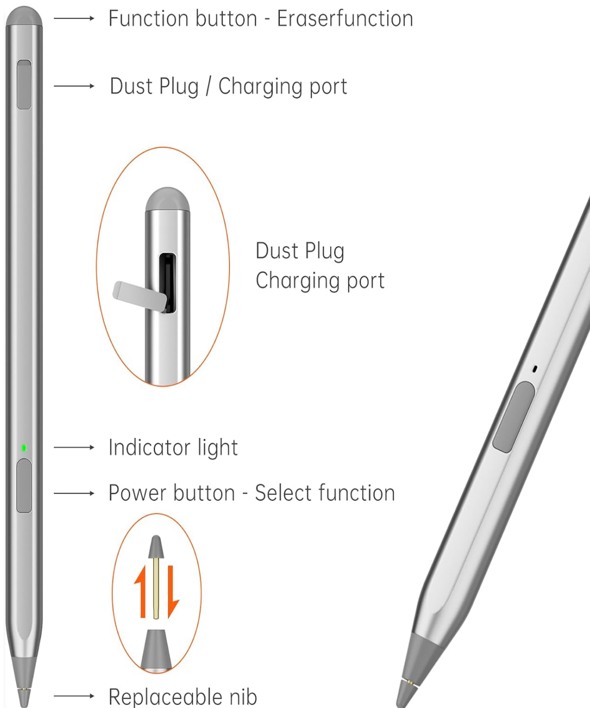
Image: Detailed diagram of the Uogic USI 2.0 Stylus Pen, highlighting its key components including the function button (eraser), dust plug/charging port, indicator light, power button (select function), and replaceable nib.
