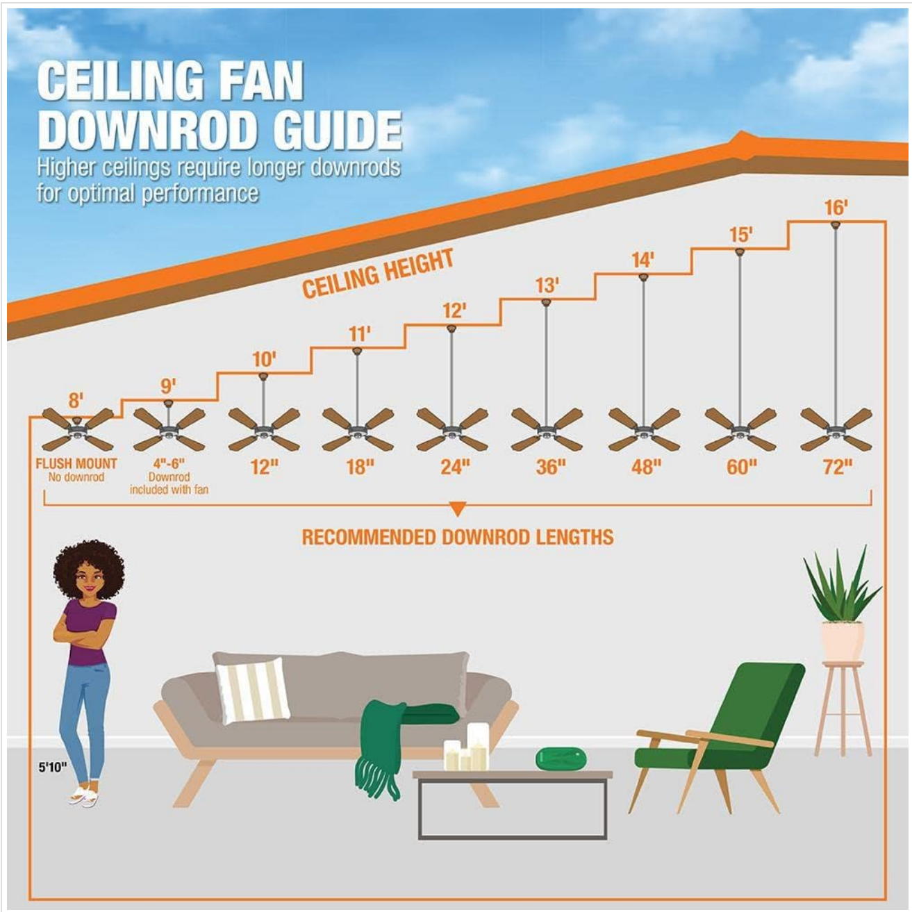
Image 4.1: Recommended downrod lengths based on ceiling height for optimal air circulation.
