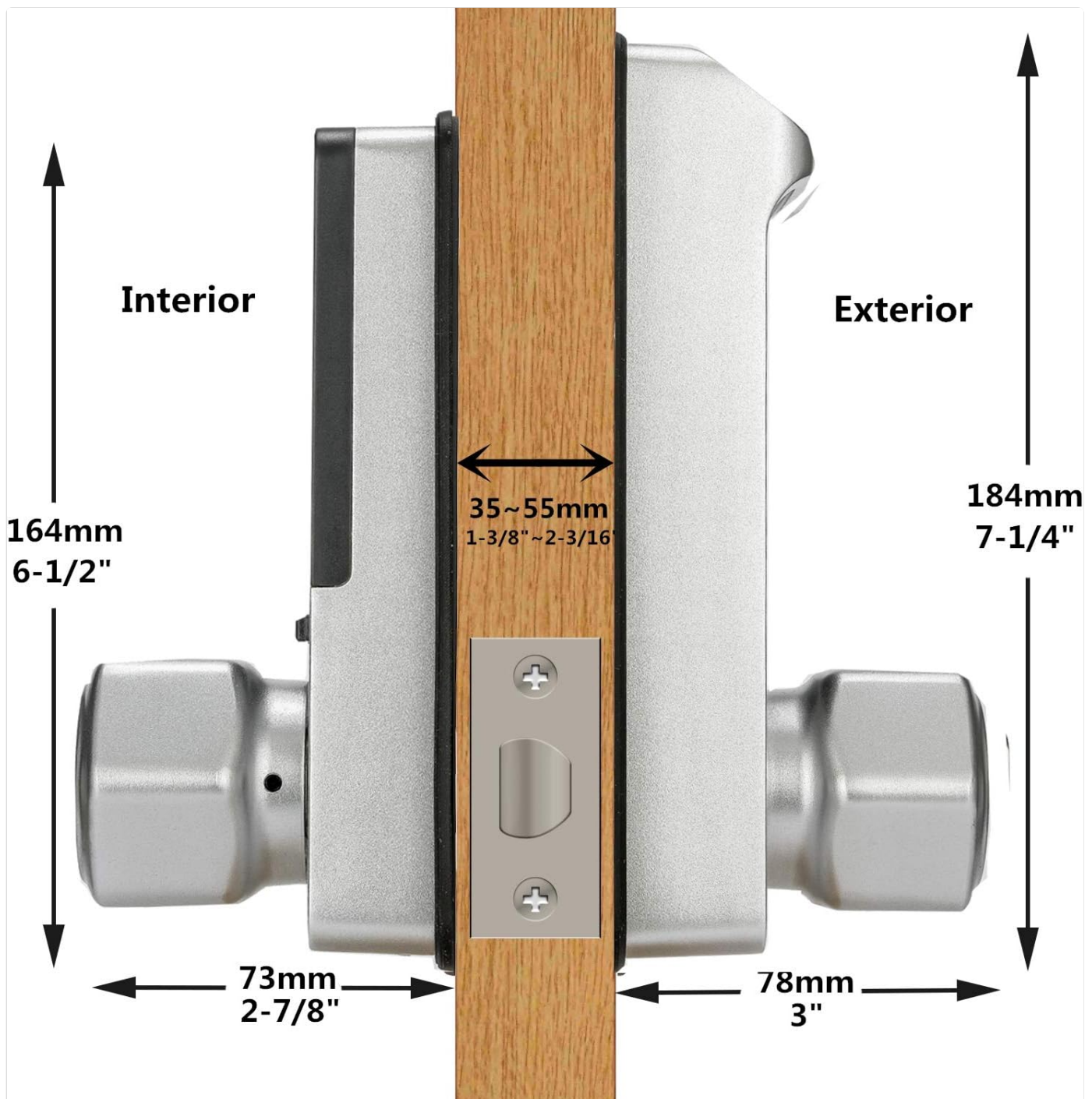
Image: Door thickness compatibility diagram, showing the required dimensions for installation.
