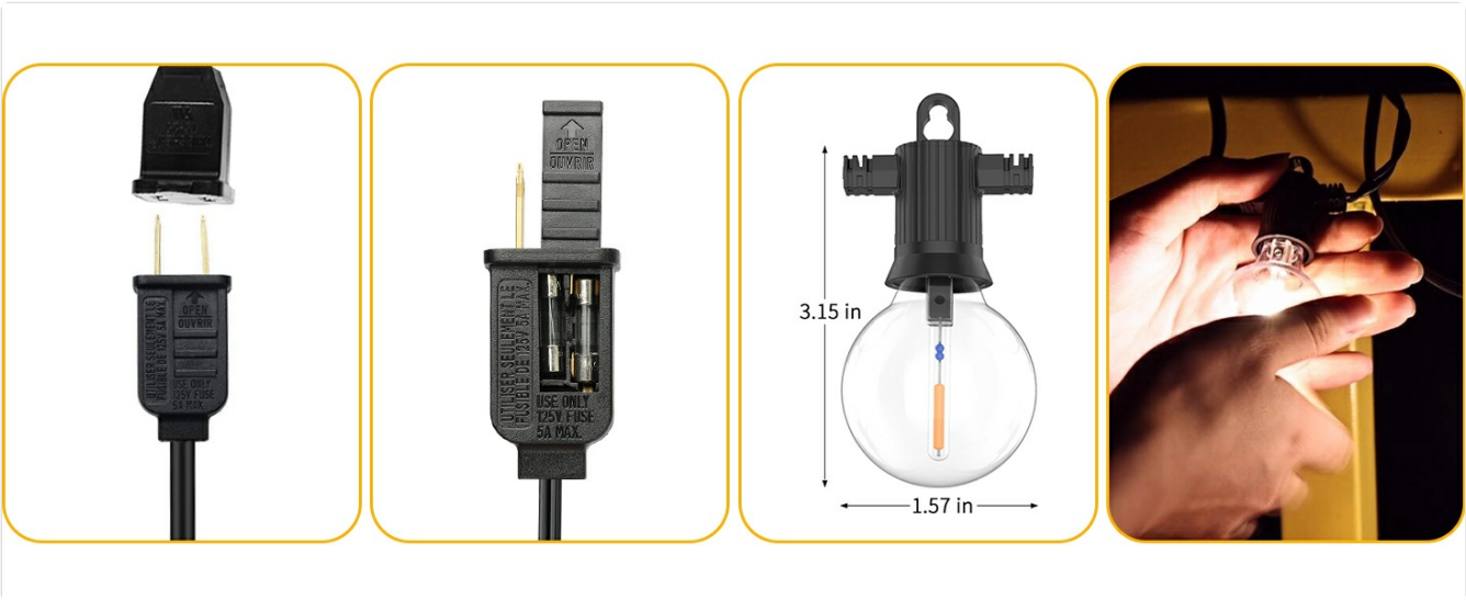
Image: Steps for connecting the power plug, accessing the fuse, and installing a bulb.
