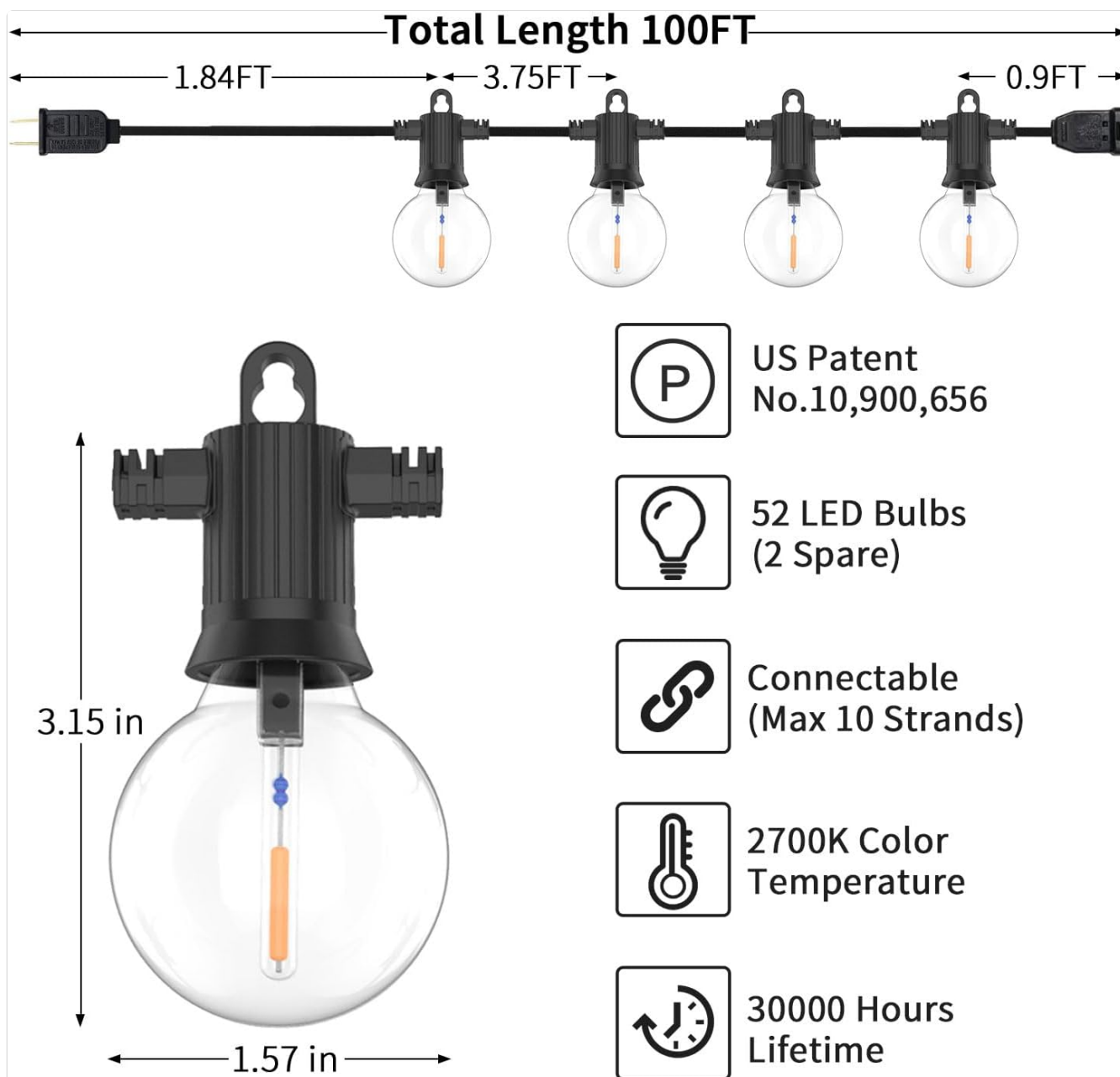
Image: Detailed dimensions and key specifications of the ZOTOYI G40 string lights.
