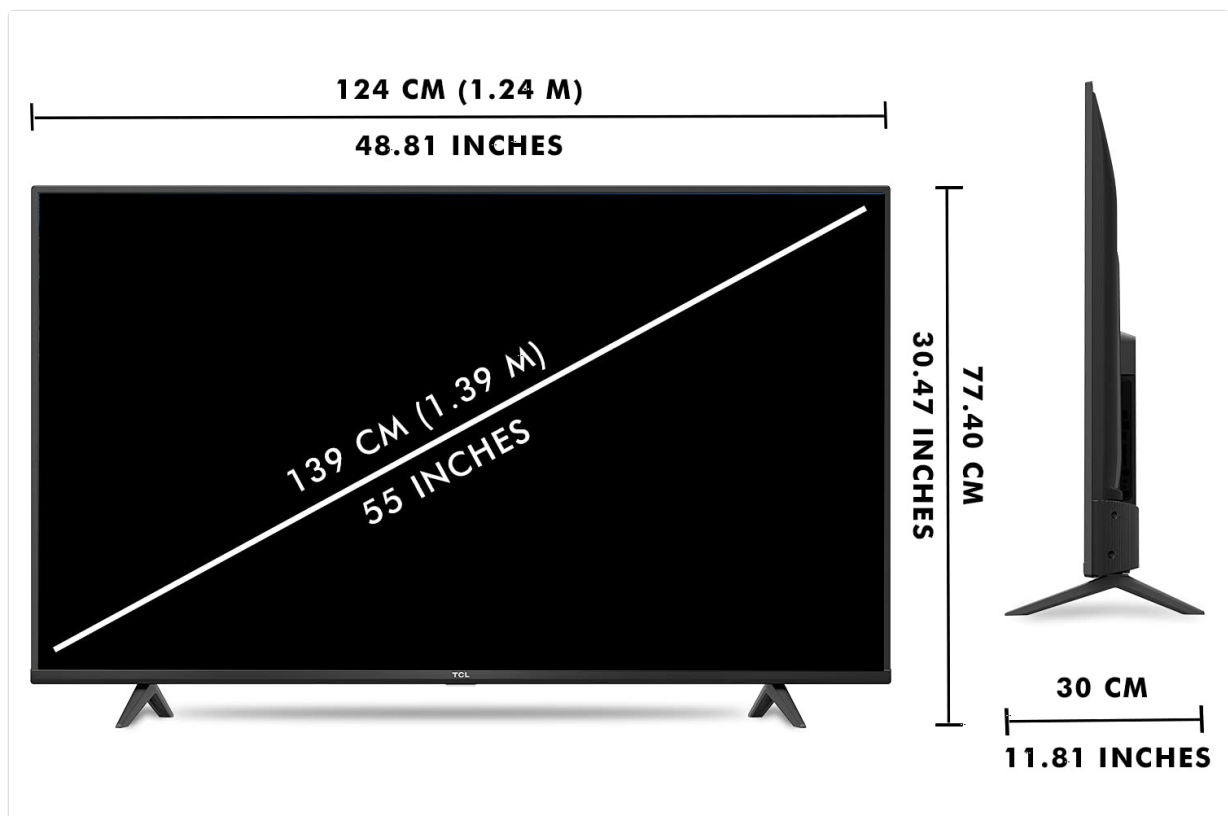
Image 11.1: Physical dimensions of the TCL 55P615 television, including screen diagonal, width, height, and depth with stand.
