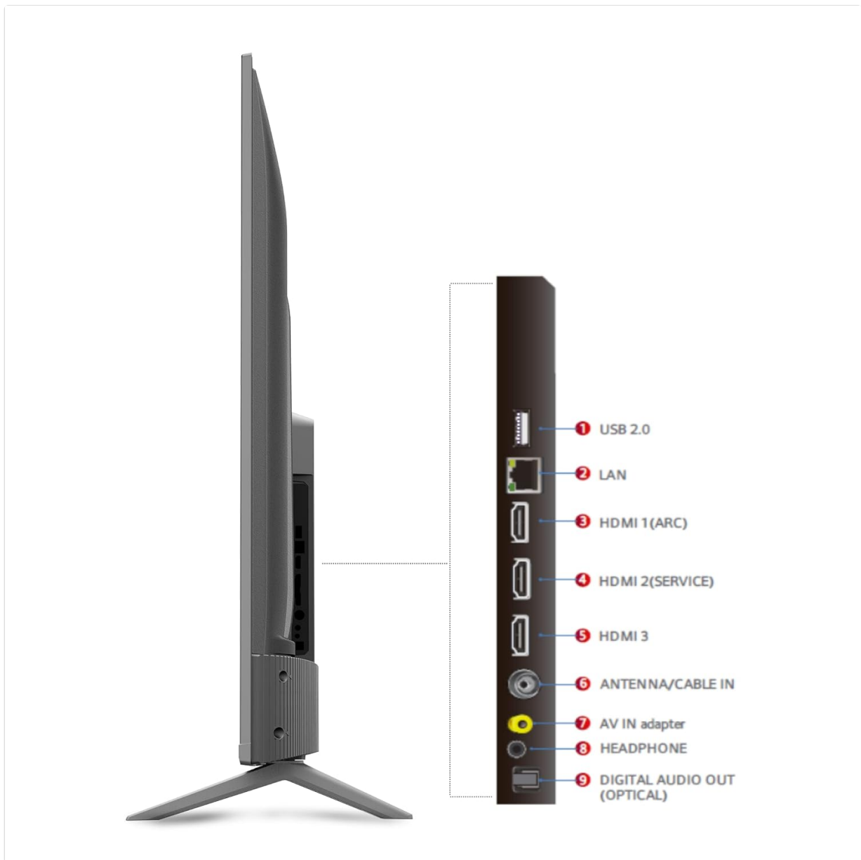
Image 4.2: Side profile of the TCL 55P615 TV with a detailed view of its various input and output ports.
