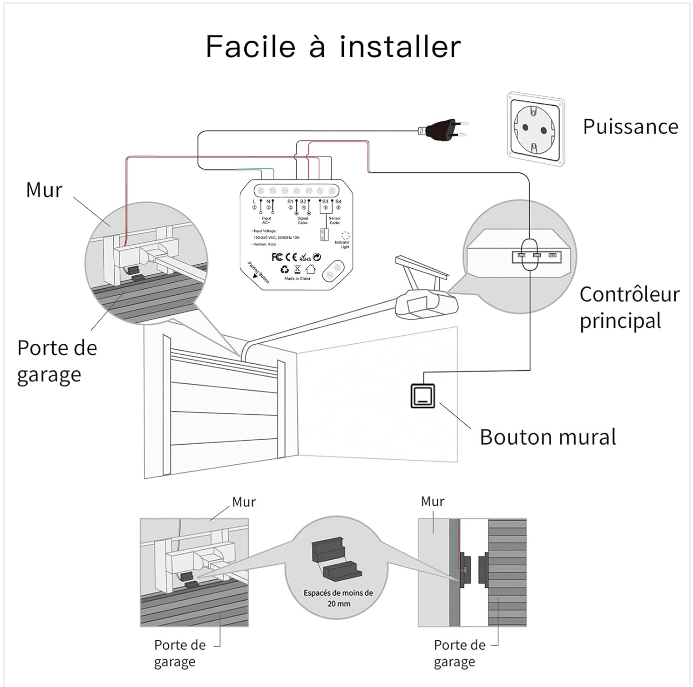
Figure 4.2: Installation Diagram. Illustrates connections for power, main controller, wall button, and door sensors, with sensor placement details.
