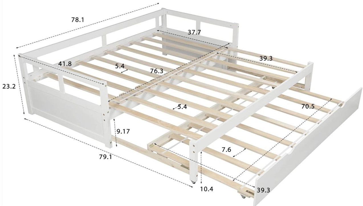
Image 8.1: Detailed dimensions of the Merax Wooden Daybed, including length, width, and height measurements.
