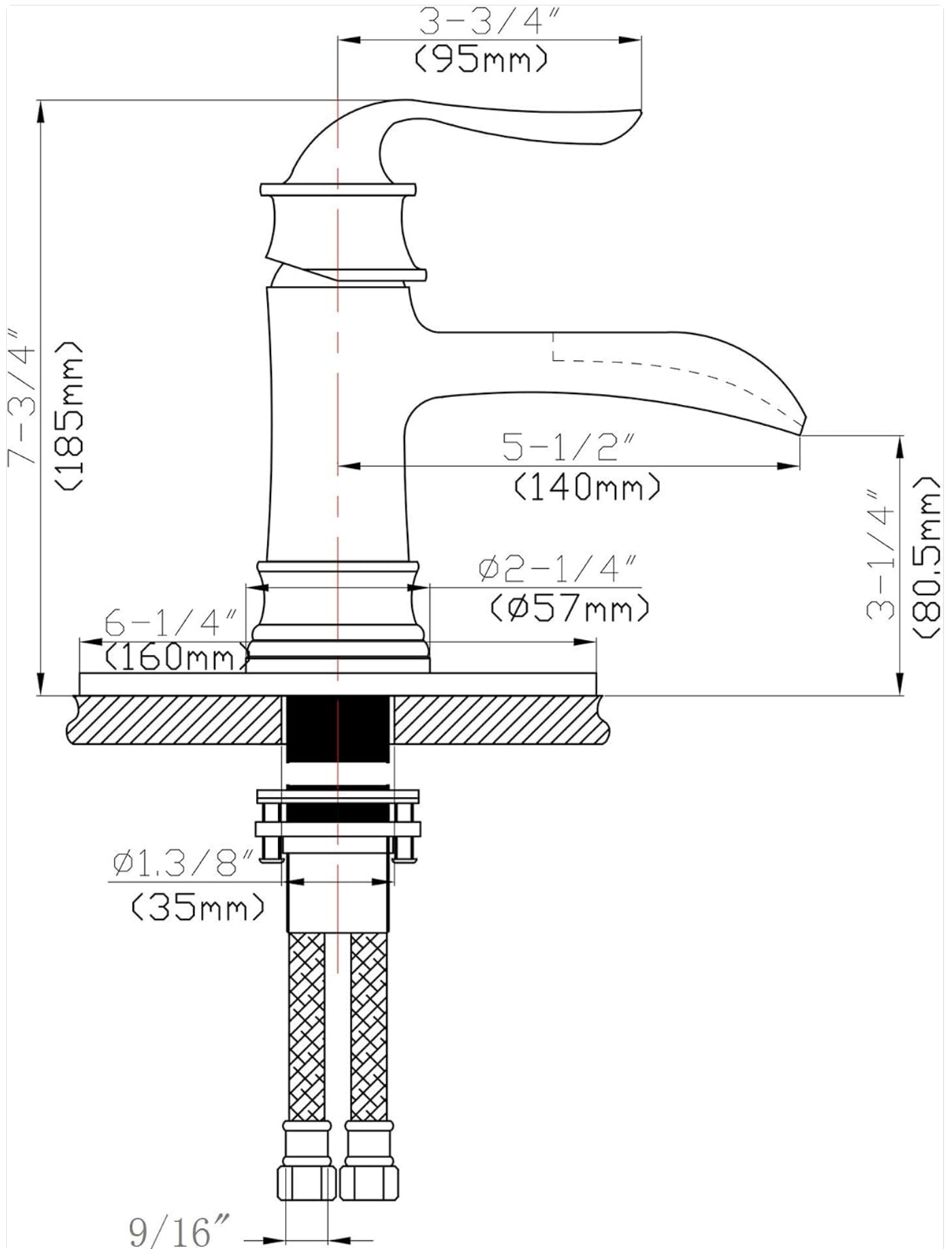
Image: Dimensional drawing of the faucet for installation planning.
