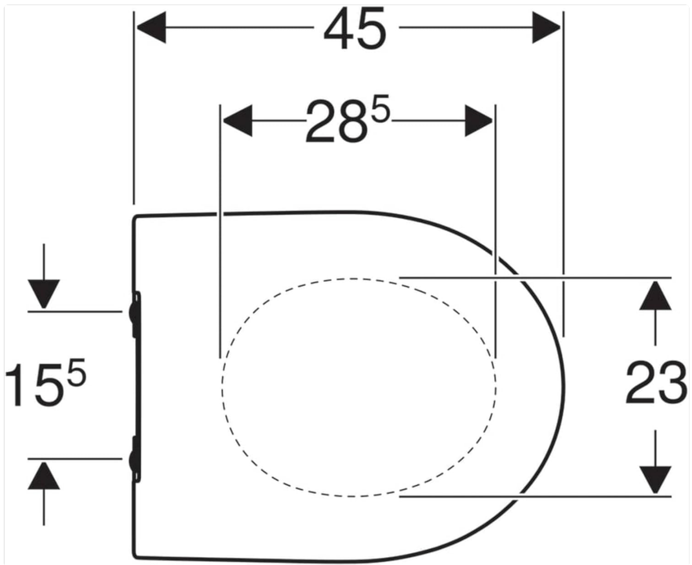
Figure 4: Top View Mounting Dimensions
