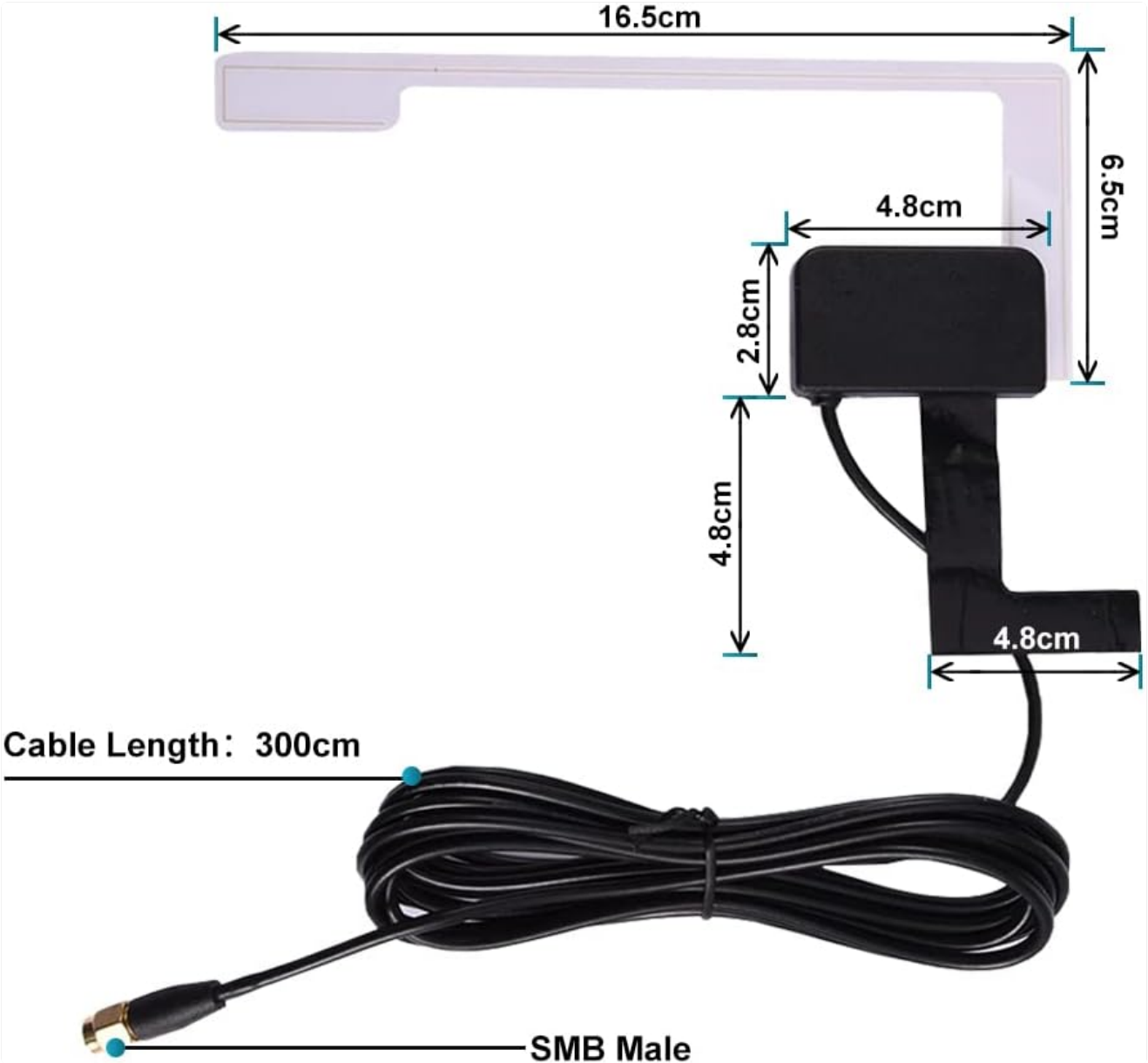
Image: Detailed dimensions of the DAB+ antenna, including its length, width, and cable length (300cm).
