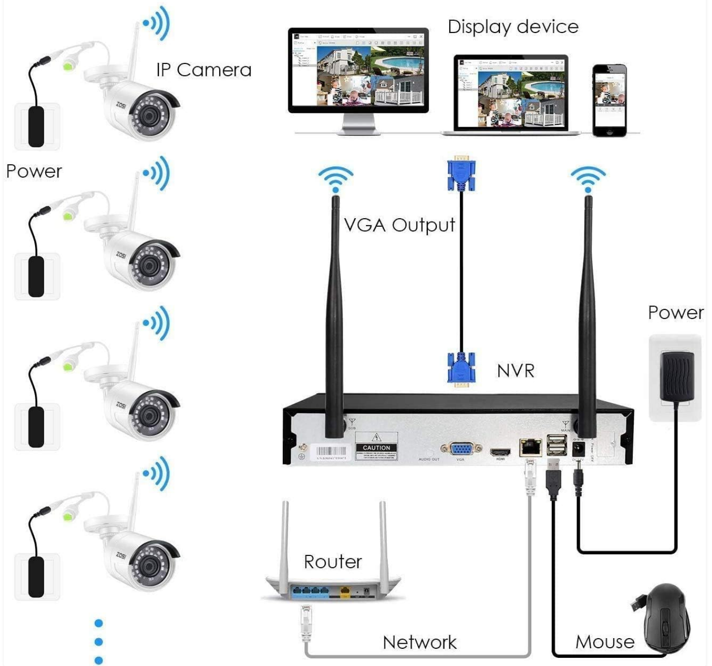
Figure 7: Overview of connecting IP cameras to the ZOSI NVR system, including power, router, and display connections.
