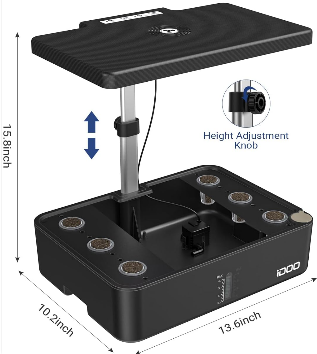
Figure 5: The adjustable height mechanism of the LED grow light, allowing for plant growth up to 11.02 inches.
