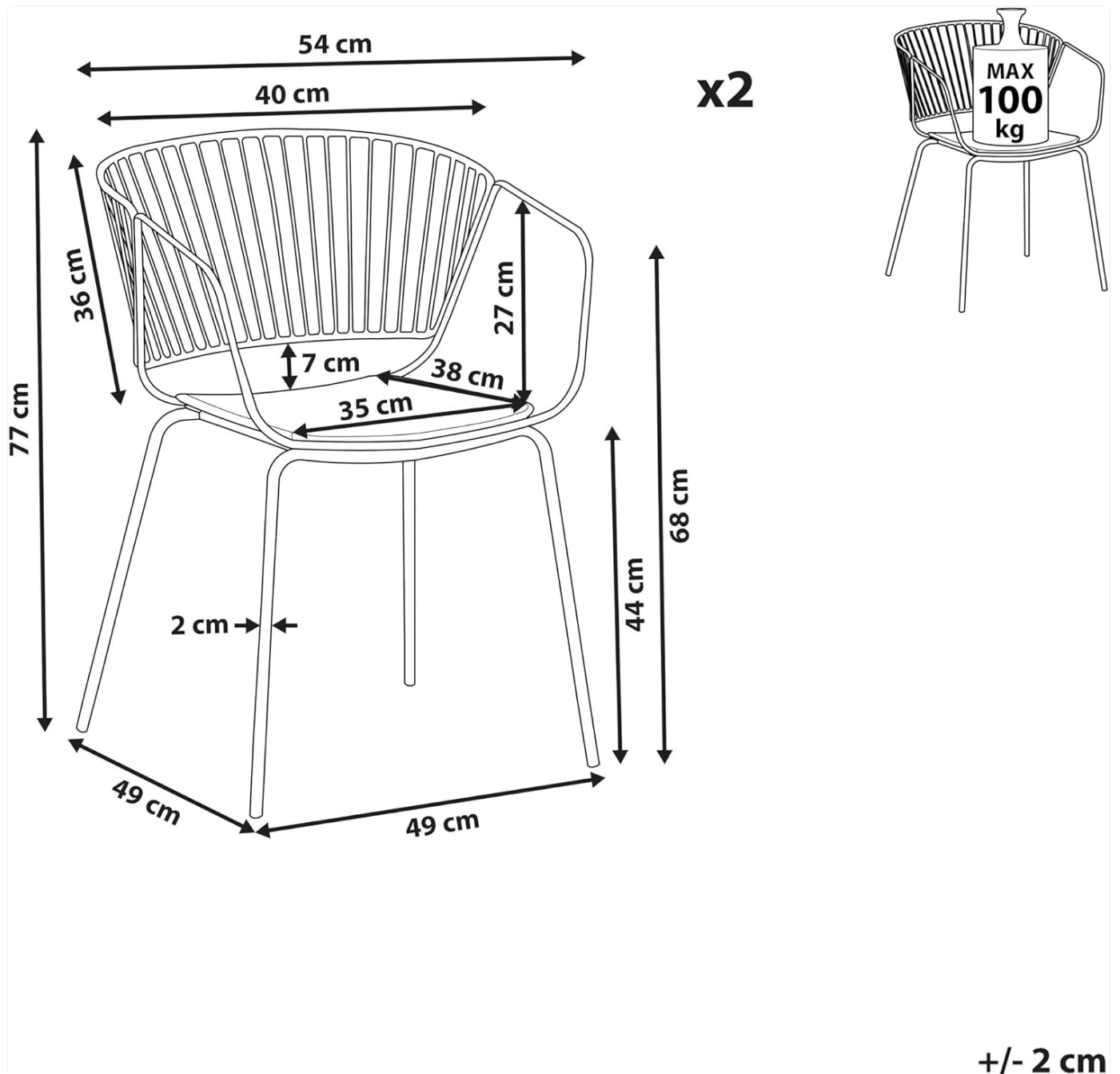
Image 7.1: Detailed dimensions of the Beliani Rigby dining chair.
