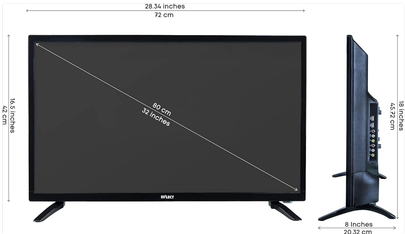
Figure 4.1: TV with table stands and dimensions.
