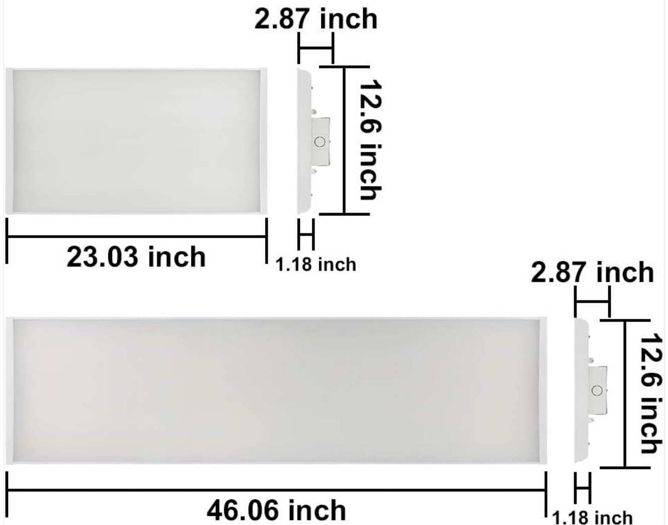
Figure 3: Dimensions for the 2-foot (23.03"L x 12.6"W x 2.87"H) and 4-foot Konlite Linear High Bay Lights.
